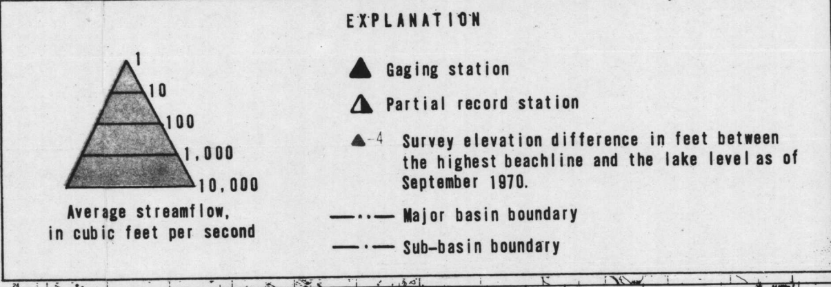
Plate 2.--Surface-water basins: hydrographs of seasonal and year-to-year maximum, minimum, and mean discharge, Kenai and Kaslof Rivers and Beaver Creek; and table showing summary of surface-water gaging-station and partial records.
