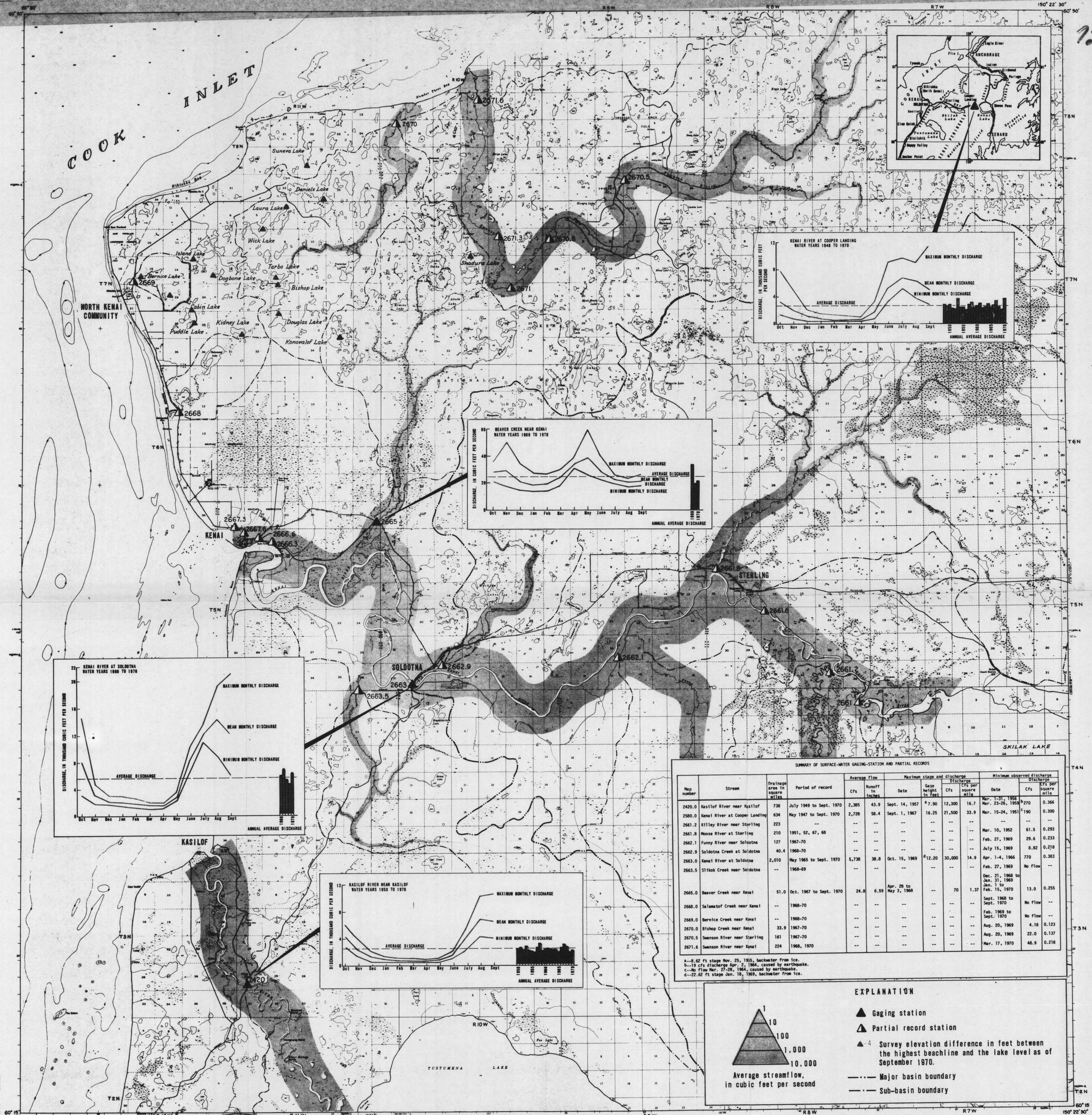
Plate 2.--Surface-water basins: hydrographs of seasonal and year-to-year maximum, minimum, and mean discharge, Kenai and Kaslof Rivers and Beaver Creek; and table showing summary of surface-water gaging-station and partial records.
