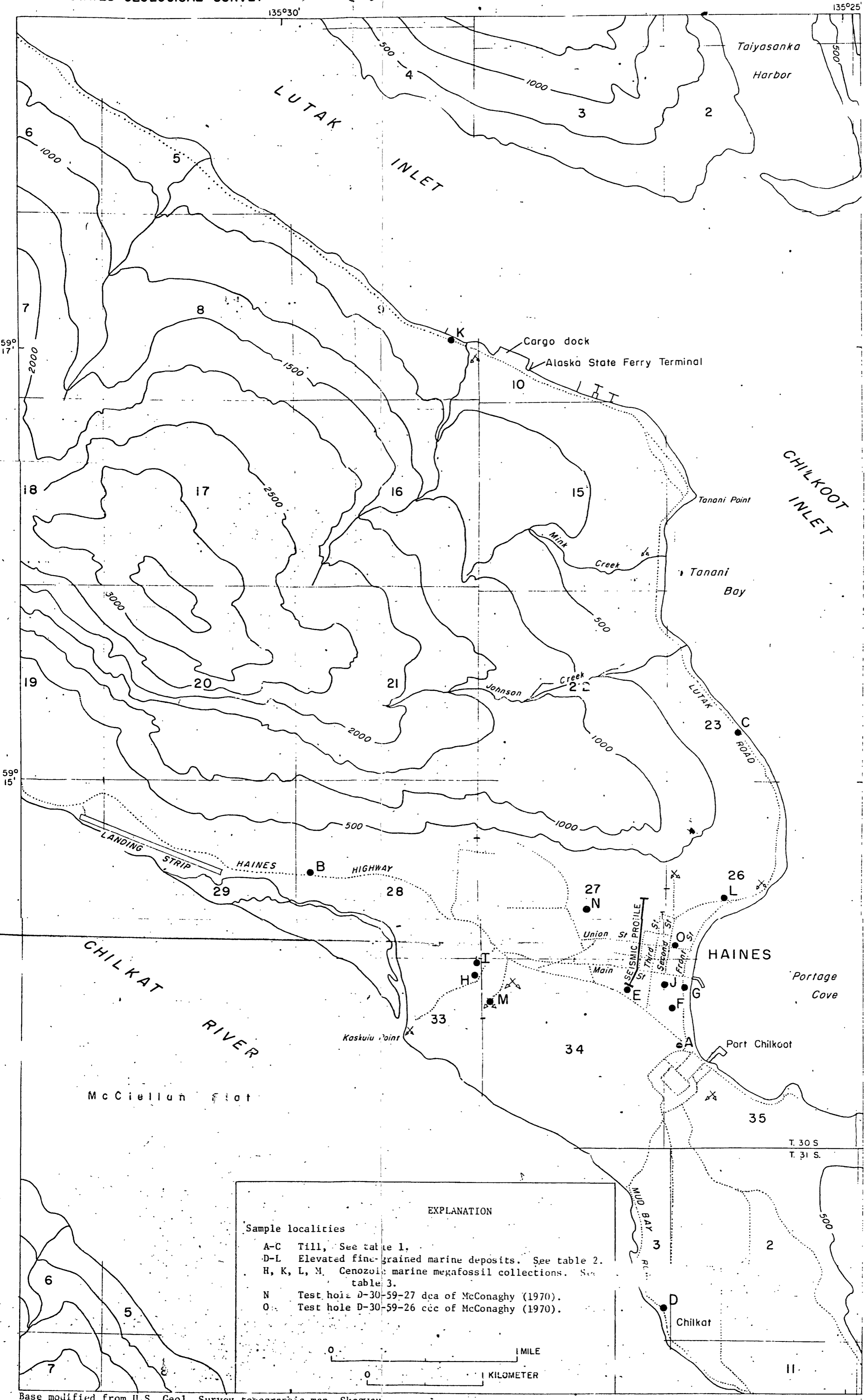
Figure 4.--Generalized map of Haines area showing sample locations, test holes, and line of seismic profile.
