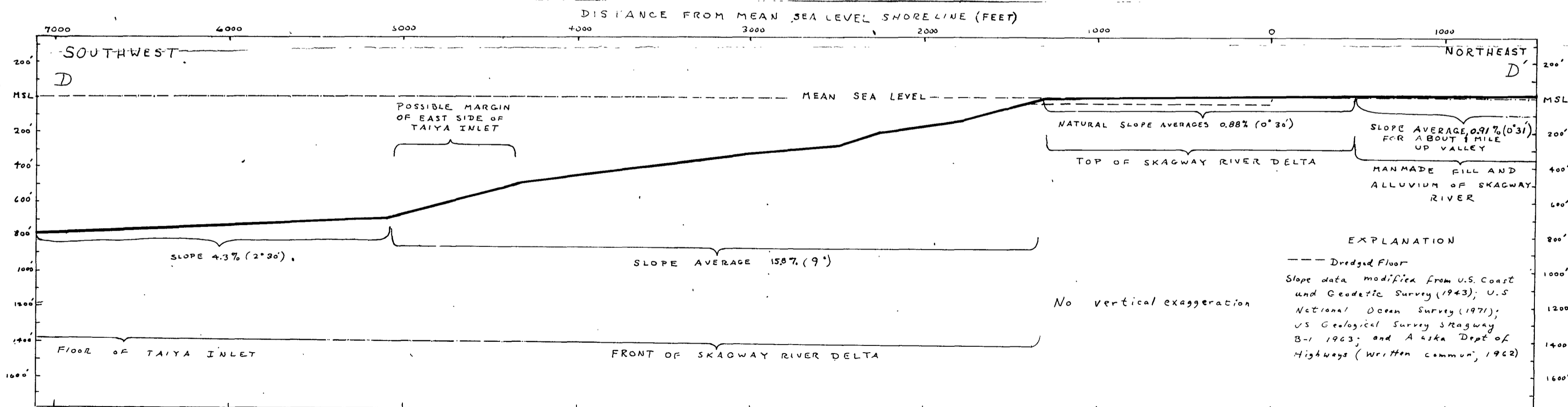
Figure 10.— Longitudinal profile D-D' along Skagway River delta and parts of Taiya Inlet and lower Skagway valley, Alaska. See figure 6 for location
