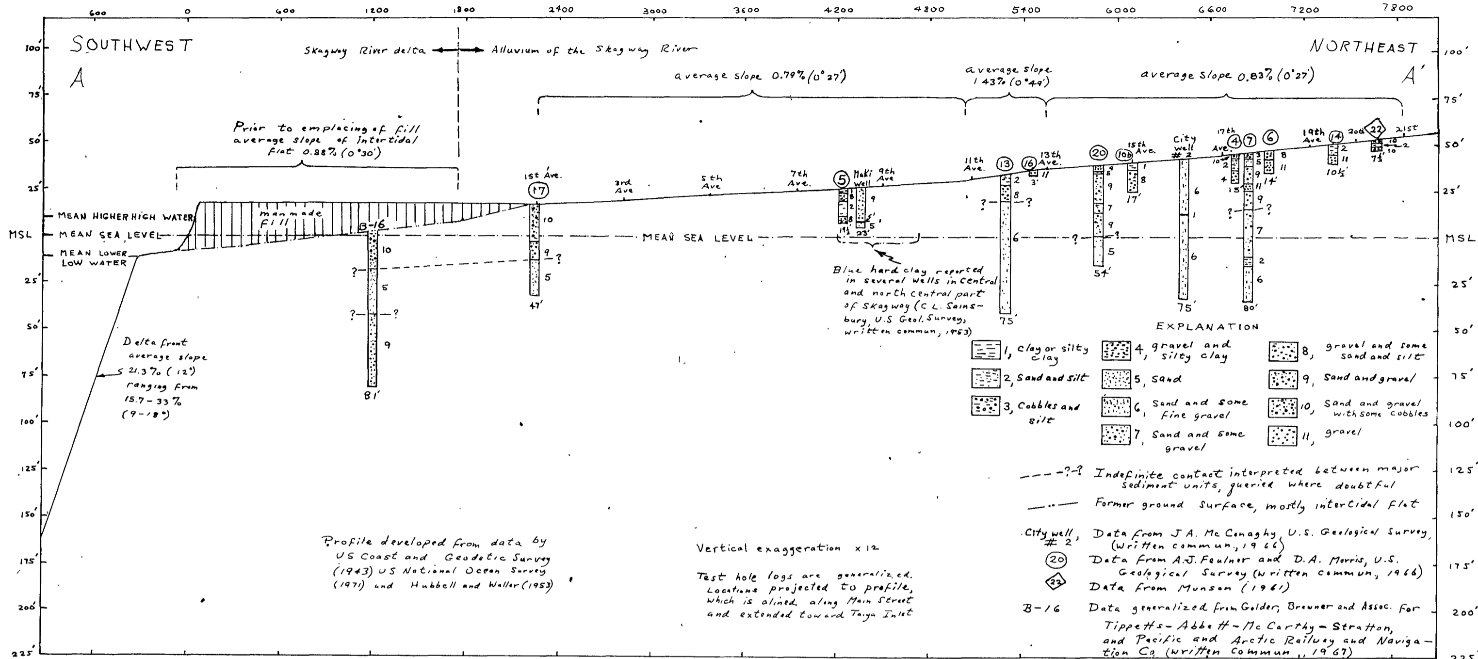
Figure 7.— Profile A-A' along part of lower Skagway valley and Skagway River delta and data from selected test holes. See figures 4 and 6 for locations
