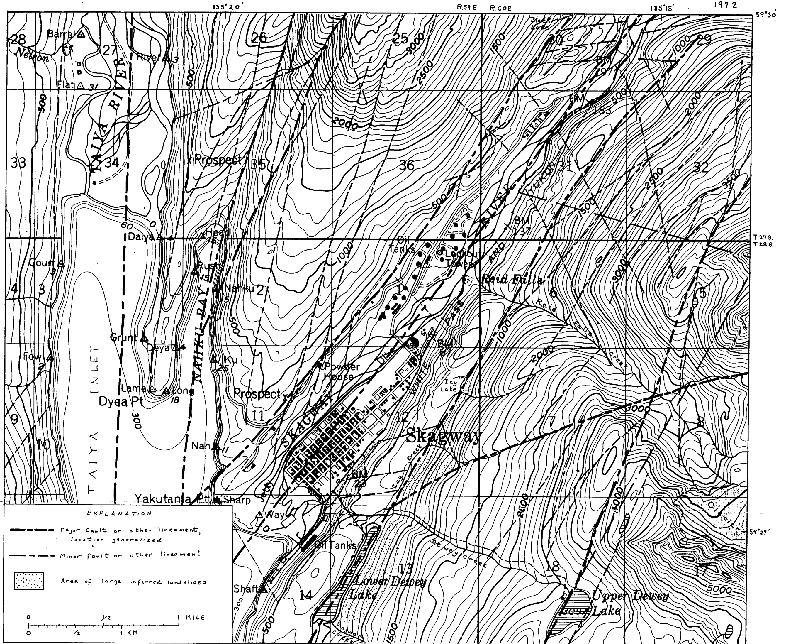
Figure 15.—Map of Skagway and vicinity, Alaska, showing faults or other lineaments and large inferred land slides. See Figure 14 for location. Base from U.S. Geological Survey Skagway B-1, 1963.
