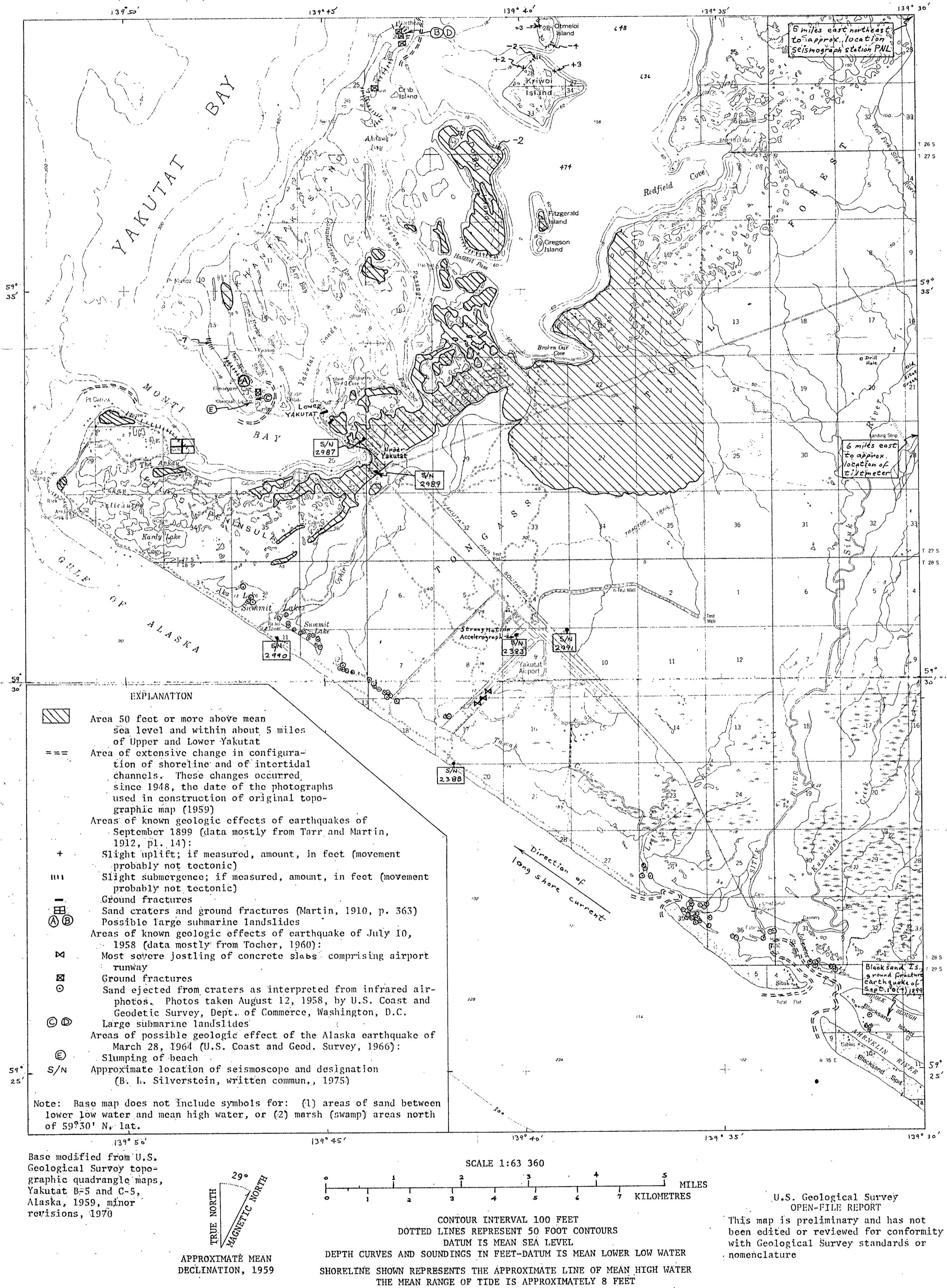
FIGURE 2.--MAP OF THE YAKUTAT AREA, ALASKA, SHOWING SELECTED TOPOGRAPHIC, HYDROLOGIC, AND EARTHQUAKE-RELATED INFORMATION.
