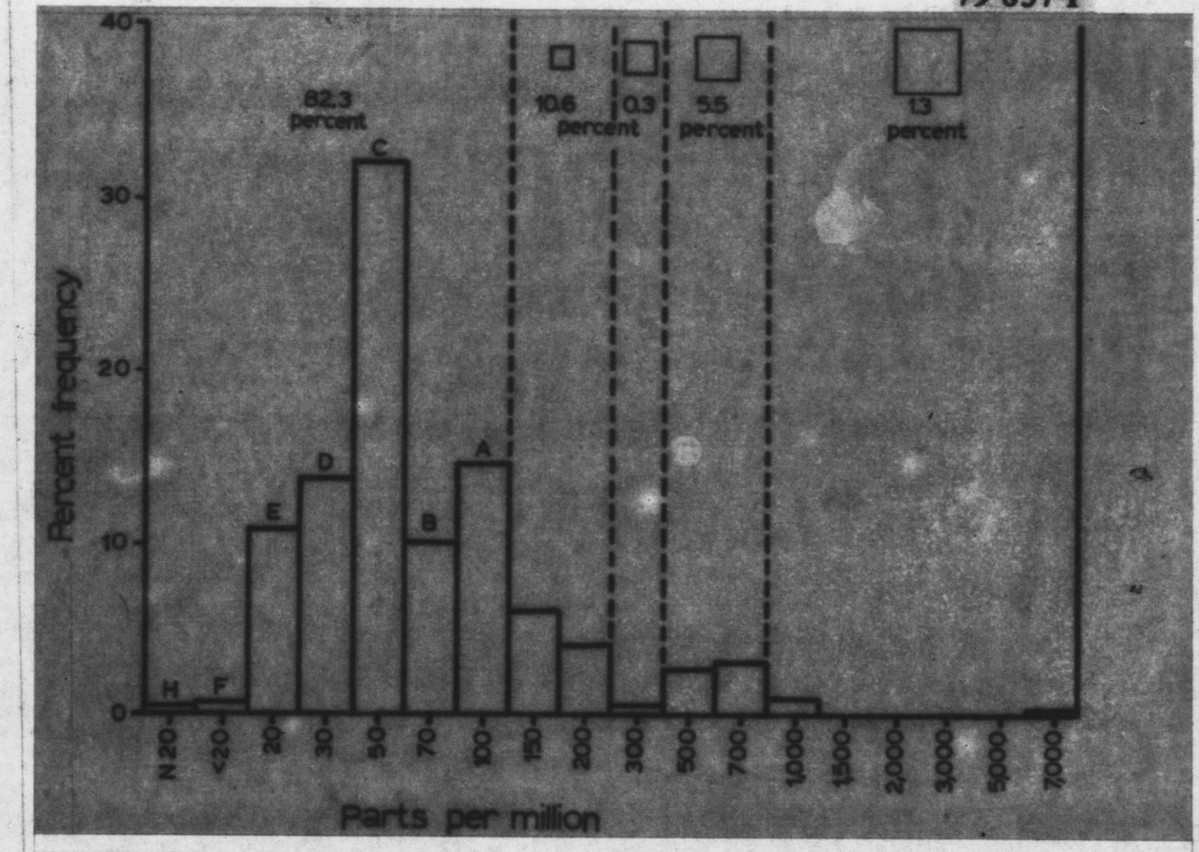
Figure 1.--Histogram for lead in 623 nonmagnetic (at >0.6 ampere) samples of heavy-mineral concentrates from stream sediments, Survey Pass 1° x 3° quadrangle, Alaska, showing map symbols corresponding to anomalous concentrations in parts per million, percentage of total samples, and letters corresponding to non-anomalous concentrations in parts per million. N, not detected at values shown; <, detected, but less than value shown. Arithmetic mean, 120; standard deviation, 322; geometric mean, 66; and geometric deviation, 2.4, based on unqualified values within the sample population.
