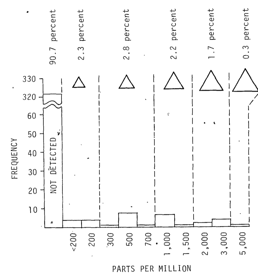
Figure 2.--Histogram for arsenic in 355 ash of aquatic-bryophyte samples, Medfra quadrangle, Alaska, showing symbols denoting concentrations and percentage of total number of samples represented by each range.
