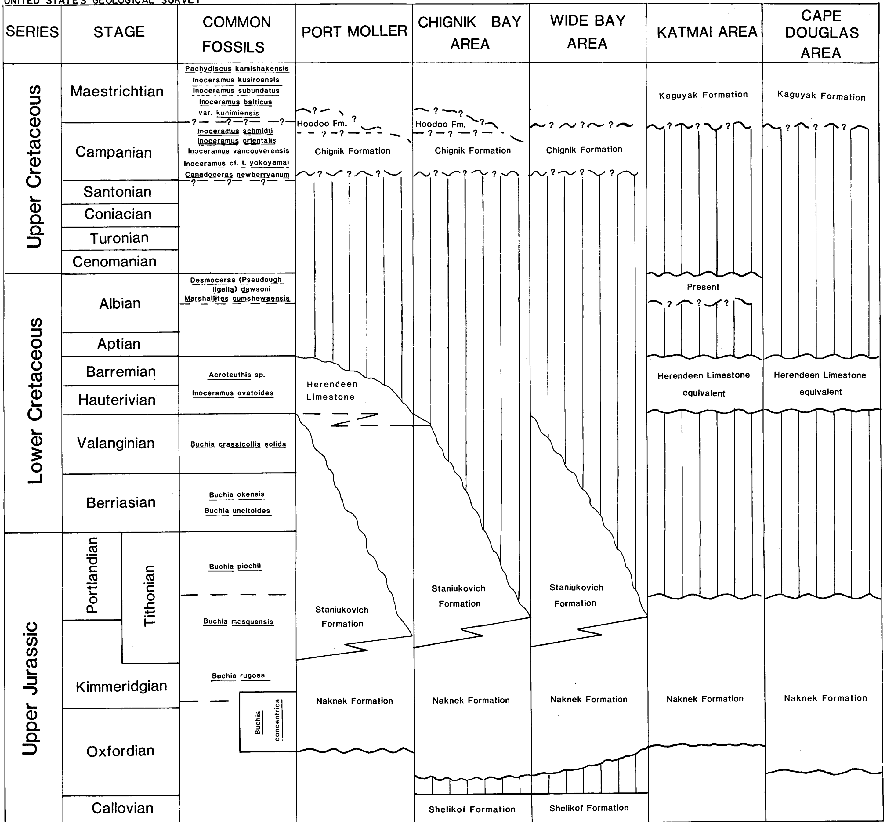
Fig. 1 Correlation chart of the Alaska Peninsula. (Burk, 1965; Imlay and Detterman, 1974; Jones, 1963) A FIELD GUIDE TO SOME COMMON MEGAFOSSILS FROM POST-CALLOVIAN MESOZOIC ROCKS OF THE ALASKA PENINSULA.
