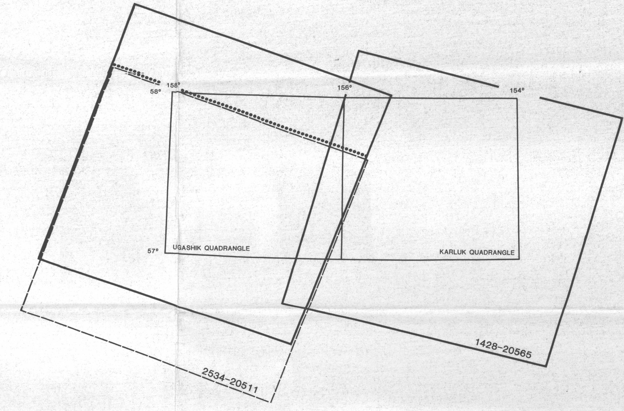
Figure 1. Map showing location of Landsat imagery used in analyses of the Ugashik and Karluk quadrangles. Dotted line indicates restricted boundary for composite image (unrelated natural color #1) noted in "Table of Imagery Used in Analyses".
