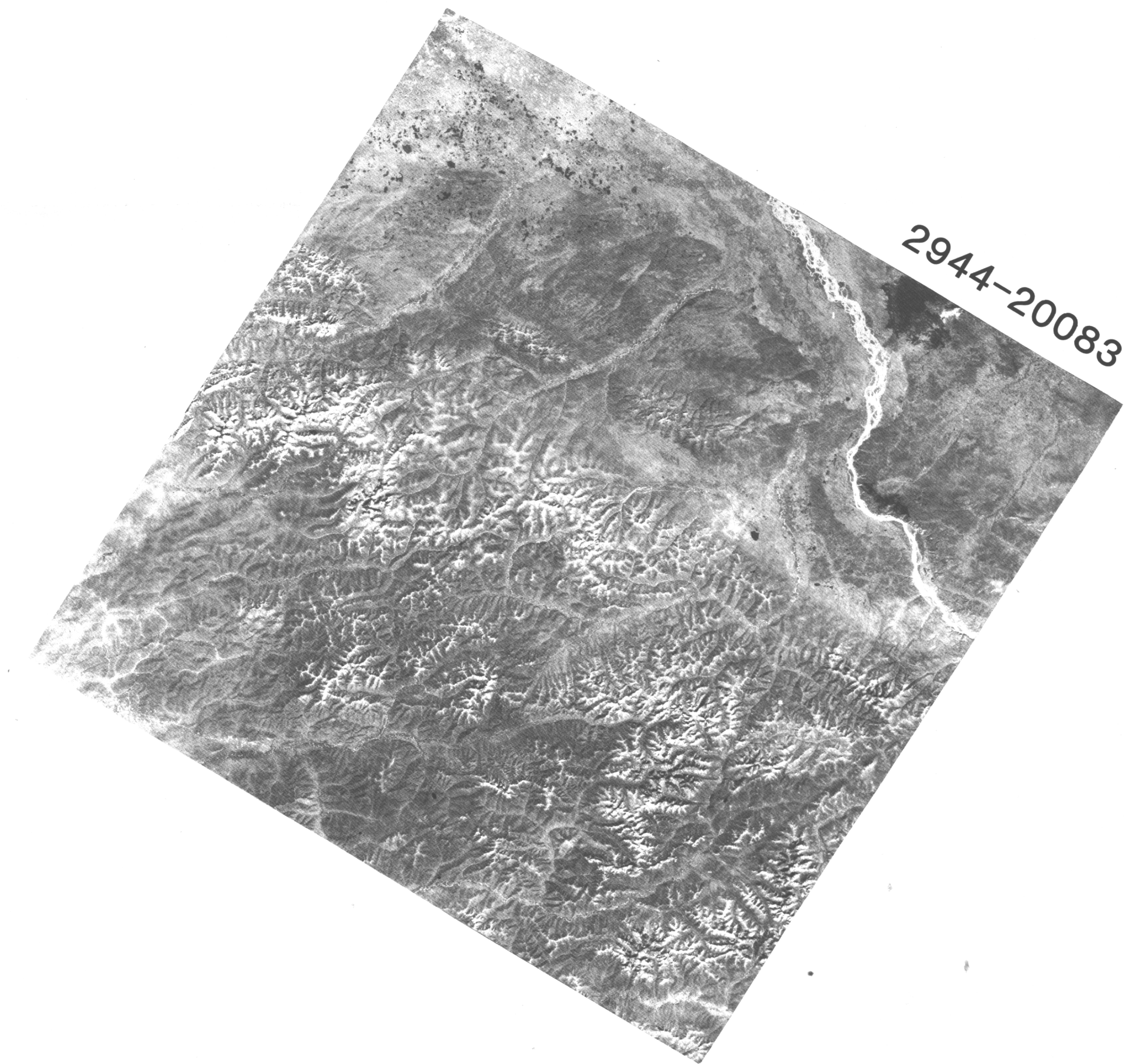
Figure 2. Example of Landsat imagery used in observations of the Circle quadrangle. Band 7.
