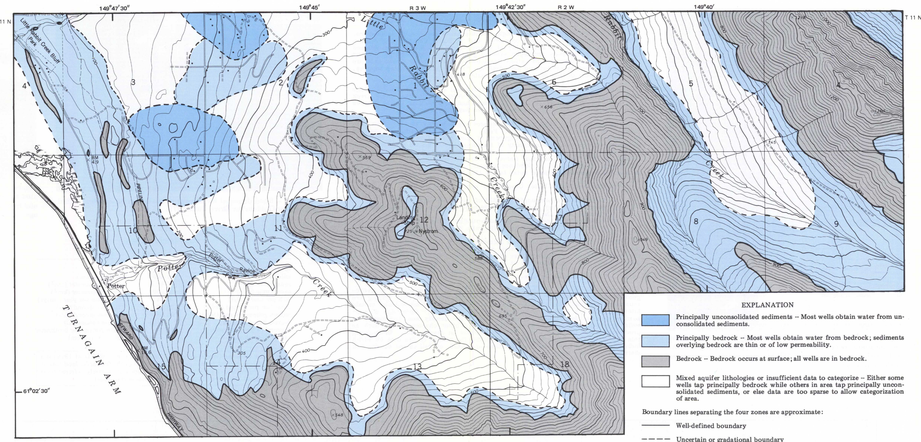
FIGURE 10. -- AQUIFER LITHOLOGY.
