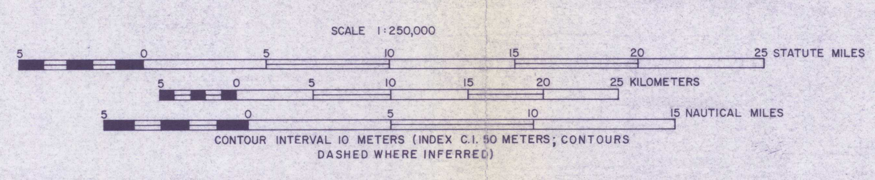
ISOPACH MAP OF HOLOCENE SEDIMENT ON THE OUTER CONTINENTAL SHELF BETWEEN YAKUTAT BAY AND DRY BAY, EASTERN GULF OF ALASKA PETER J. HOOSE, GLENN P. THRASHER AND LYNN D. LYBECK 1983
