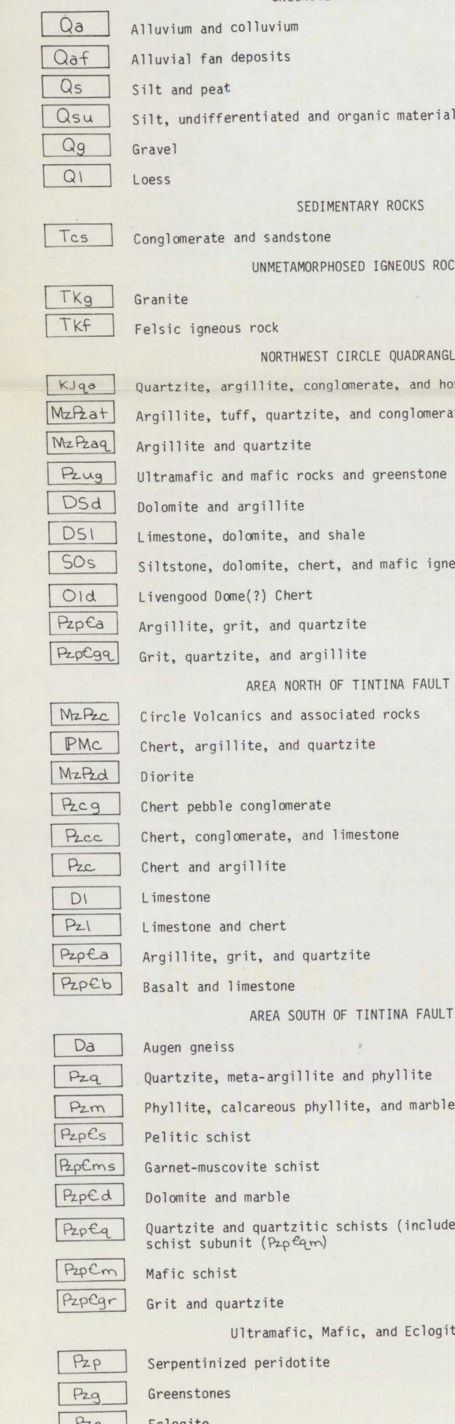
MAP H-2 MAP SHOWING DISTRIBUTION OF THE ELEMENTS Be, La, U, AND Th
