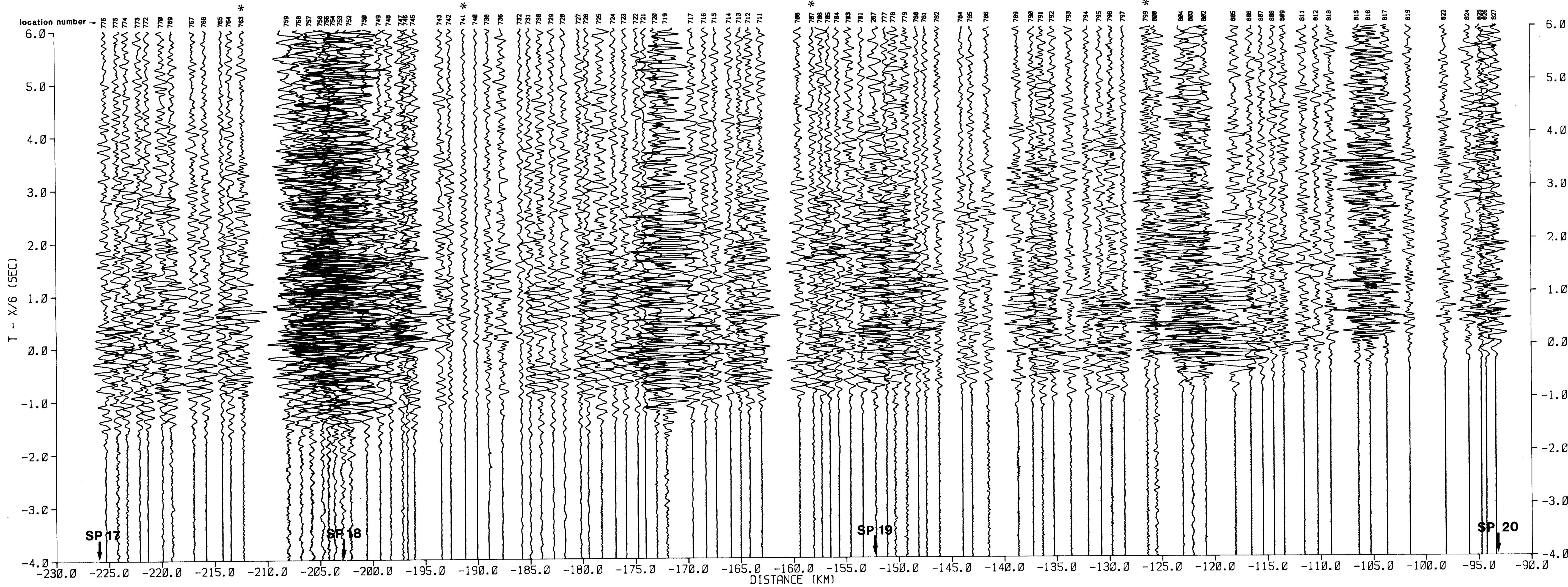
True Amplitude Record Section
