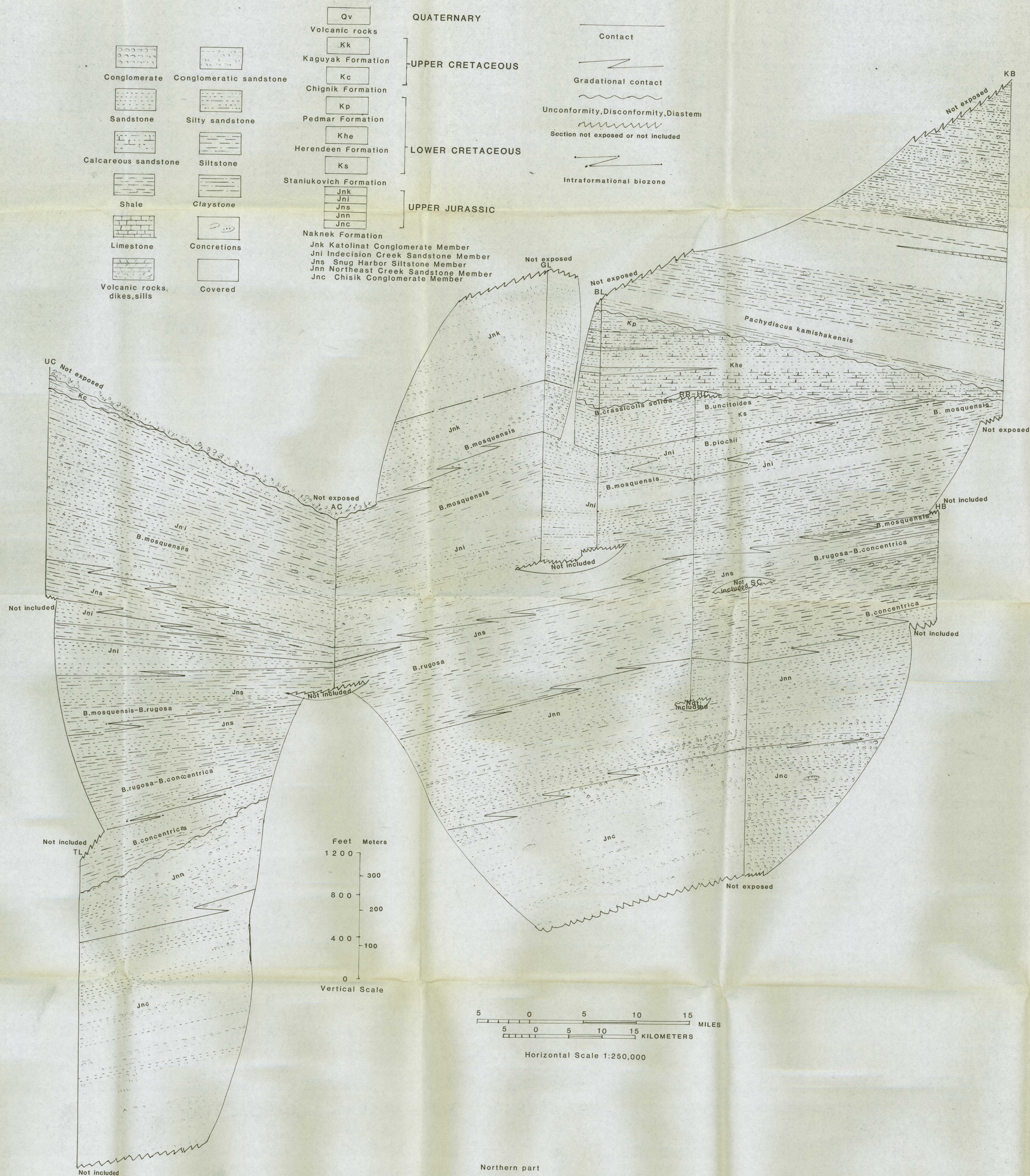
Northern part LITHOFACIES FENCE DIAGRAM OF THE UPPER MESOZOIC, ALASKA PENINSULA
