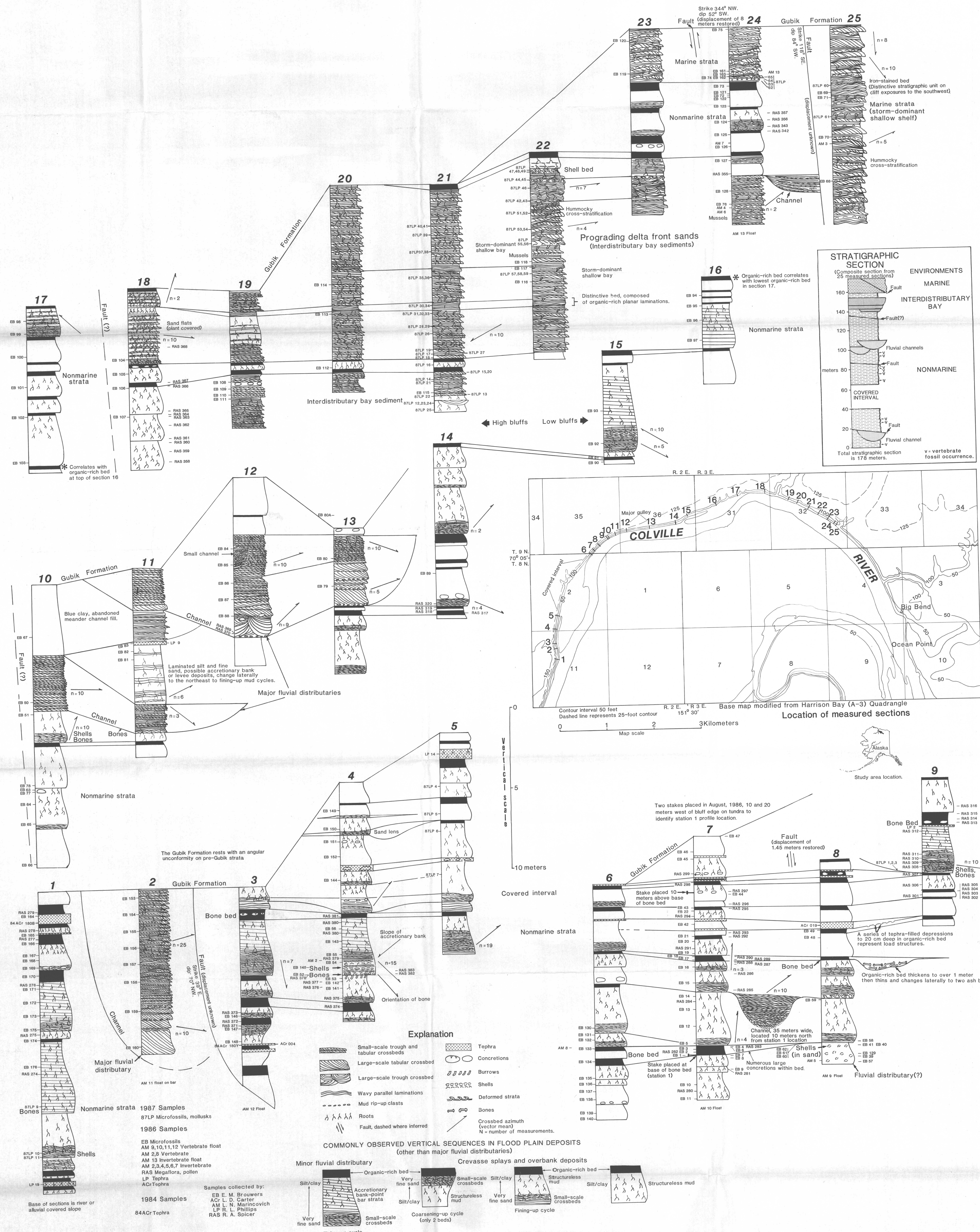
MEASURED SECTIONS, PALEOENVIRONMENTS, AND SAMPLE LOCATIONS NEAR OCEAN POINT, ALASKA
