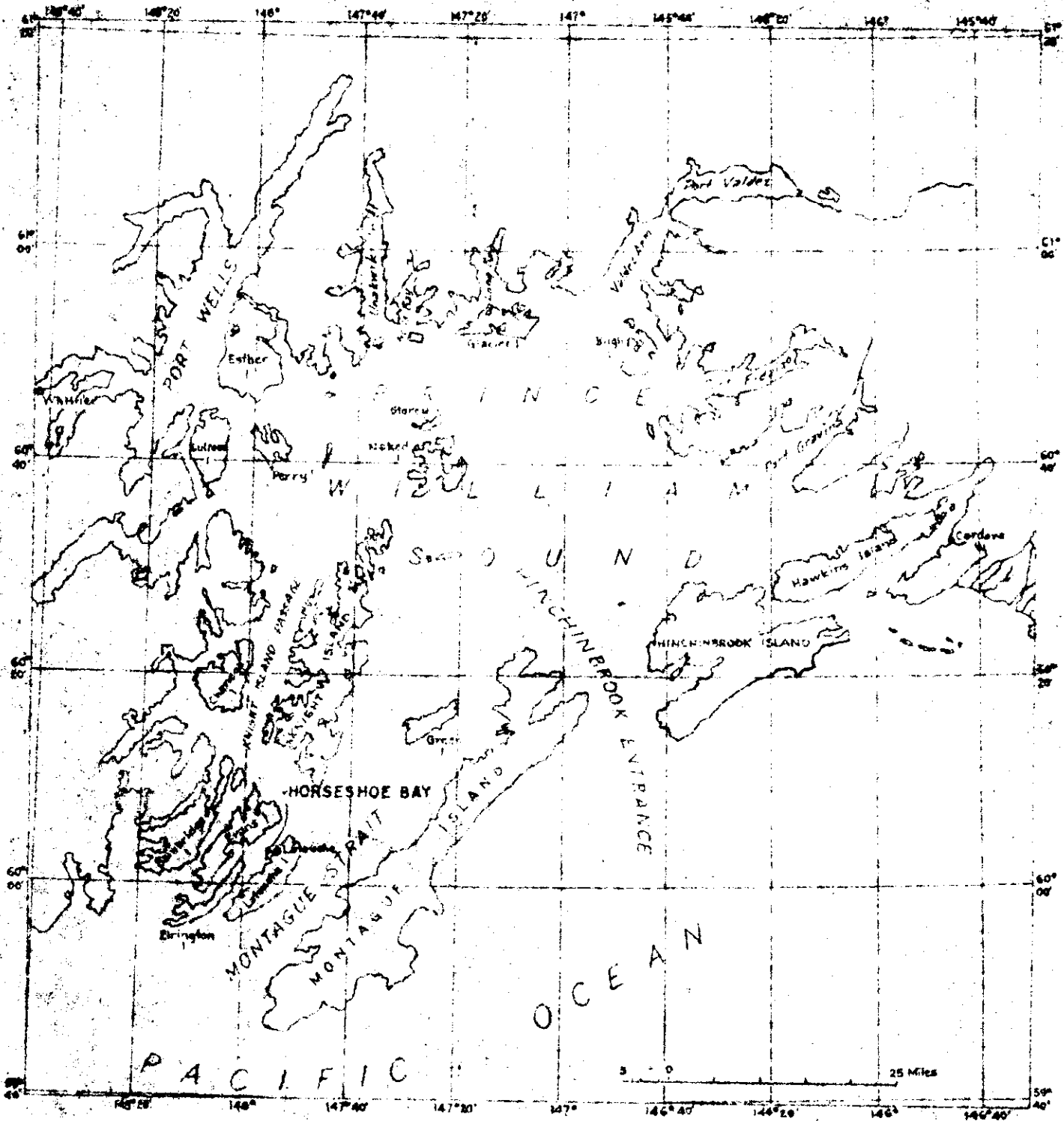
Figure 1: Index map of the Prince William Sound district, Alaska, showing location of Horseshoe Bay
