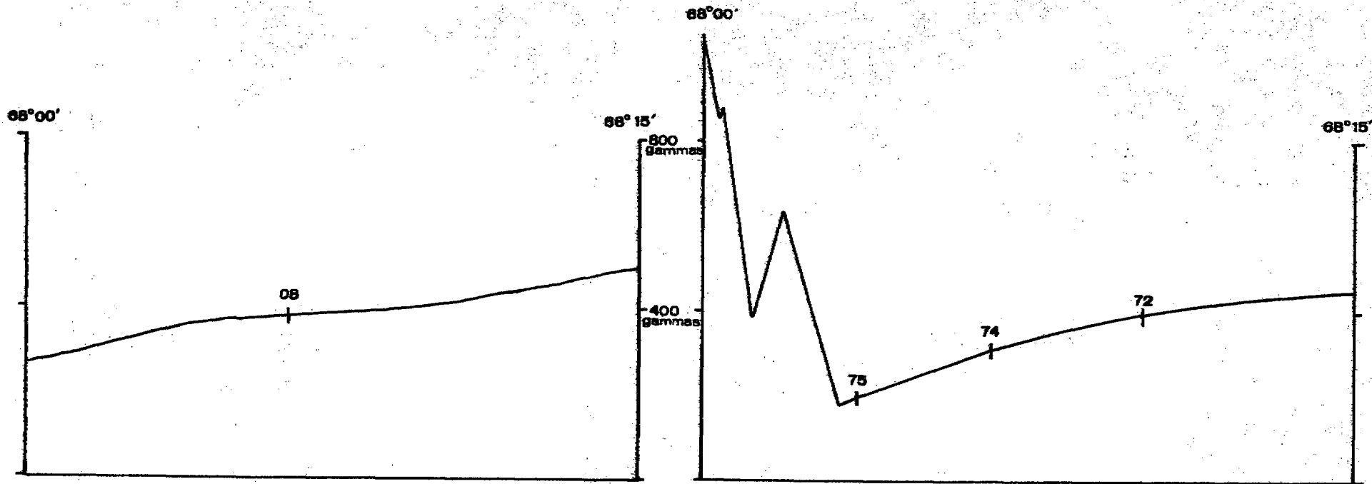
Figure 2.--Low-Altitude aeromagnetic profiles along the Wulik and Kelly Rivers as shown on Figure 1
