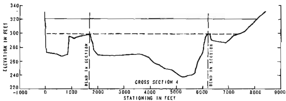
Figure 2.-- Channel cross sections, Yukon River near Stevens Village, September 1972. (Looking downstream)
