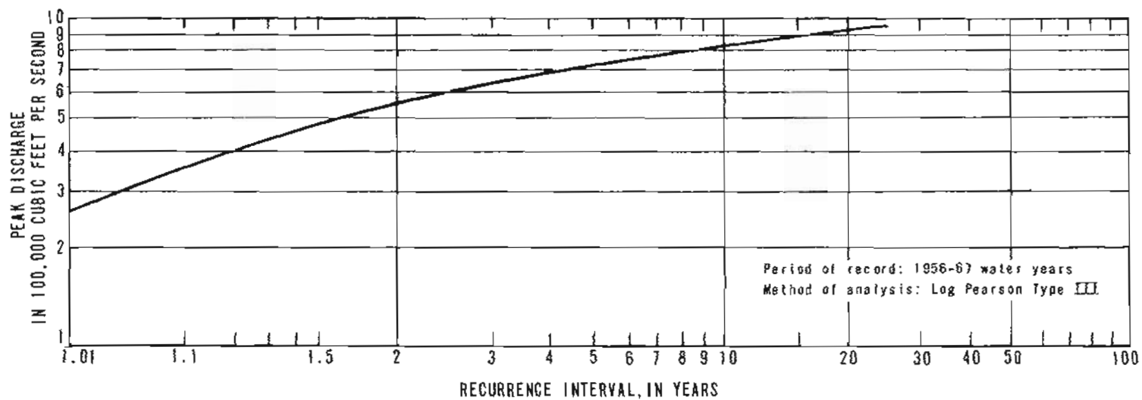
Figure 4.-- Flood magnitude-frequency relation, Yukon River at Rampart.
