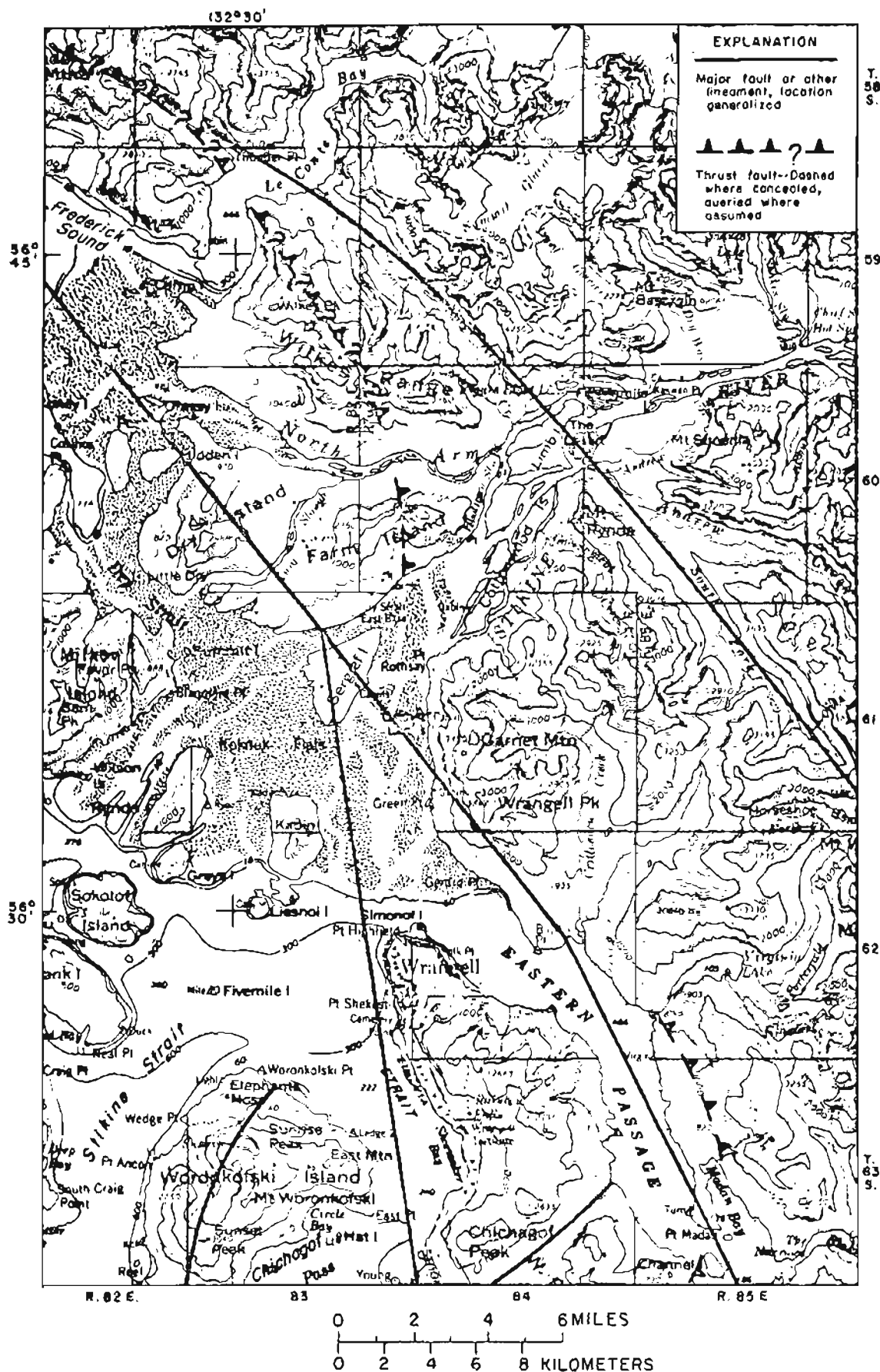
Figure 6.--Map of the Wrangell area and vicinity showing faults or other lineaments. Modified from Twenhofel and Sainsbury (1958), and Berg, Jones, and Richter (1972).
