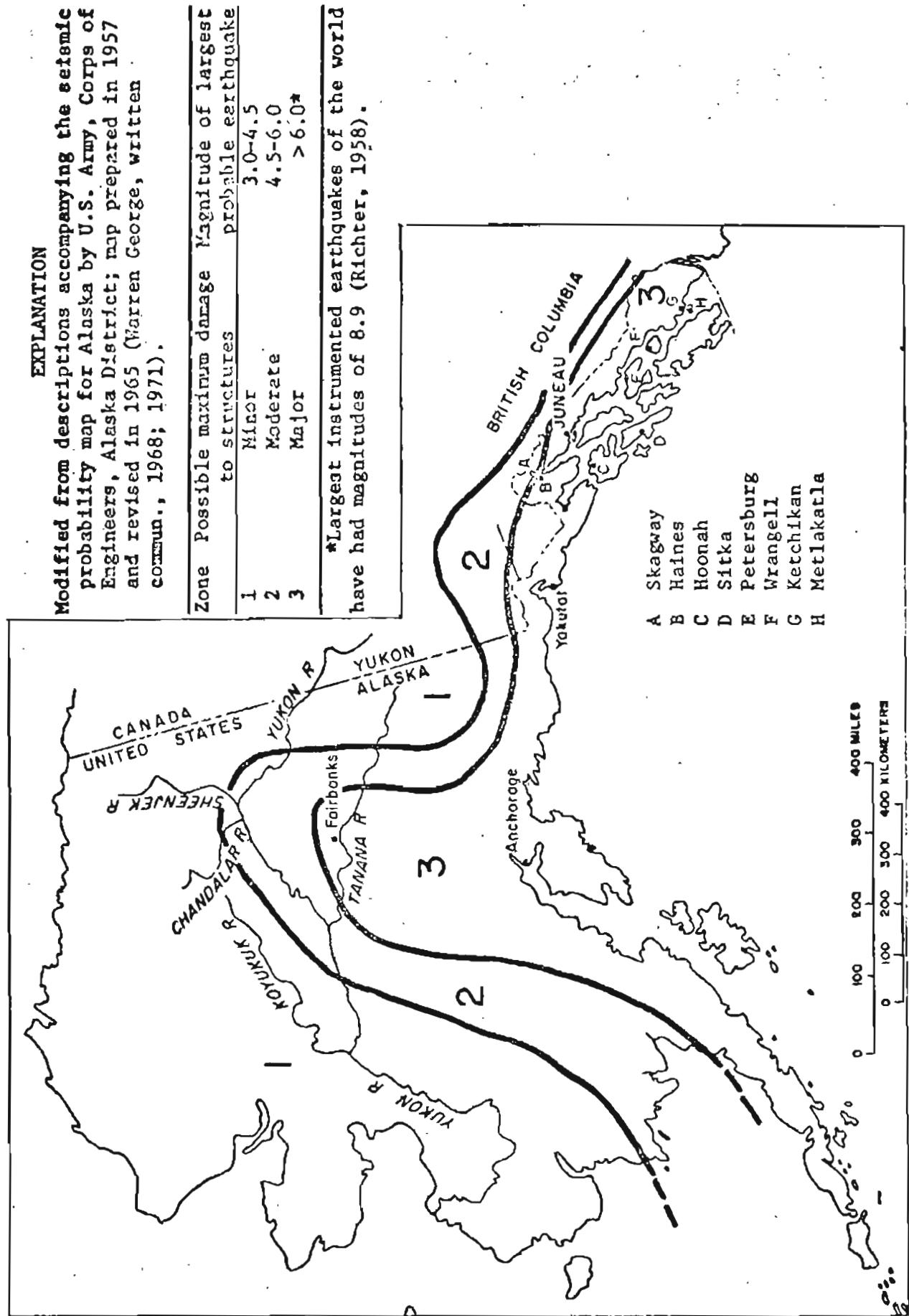
Figure 8.--Seismic probability map for most of Alaska as modified from U.S. Army Corps of Engineers, Alaska District.
