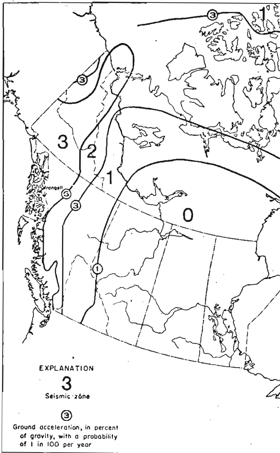
Figure 10.--Seismic zone map of western Canada. Modified from National Research Council of Canada (1970).
