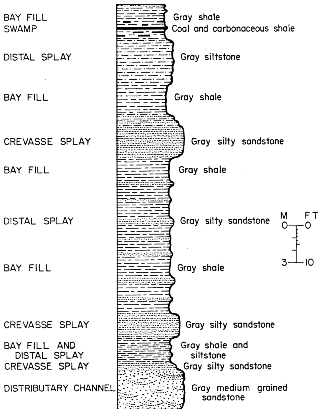
Fig. 8--Lower delta plain deposits in the Corwin Formation in SW \frac{1}{4} sec. 33, T. 1 S., R. 40 W. (Section A1078, beds 1-12).
