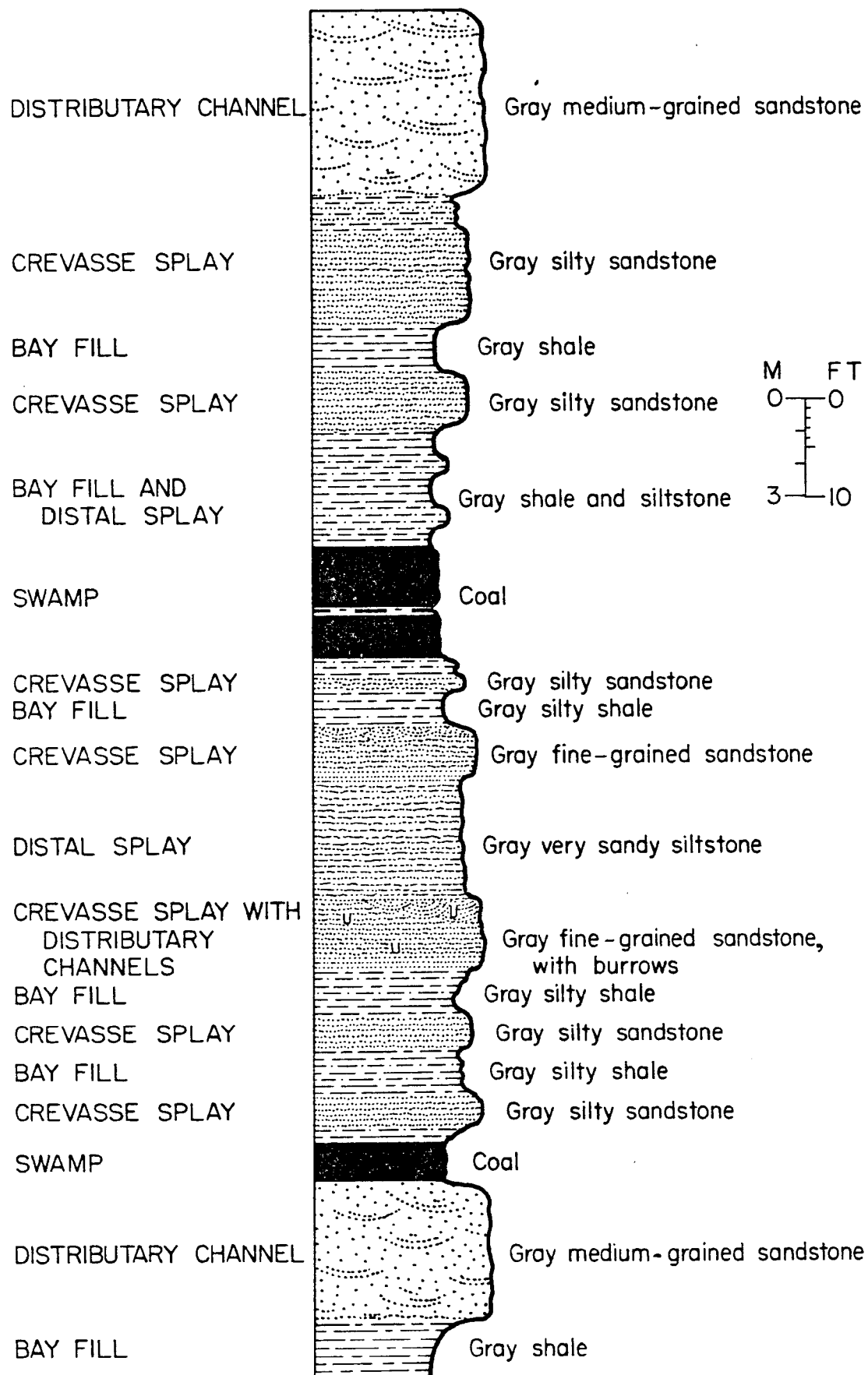
Fig. 10--Middle delta plain deposits in the Corwin Formation in NW \frac{1}{4} SW \frac{1}{4} sec. 36, T. 2 N., R. 39 W. (Section A1378, beds 6-23).
