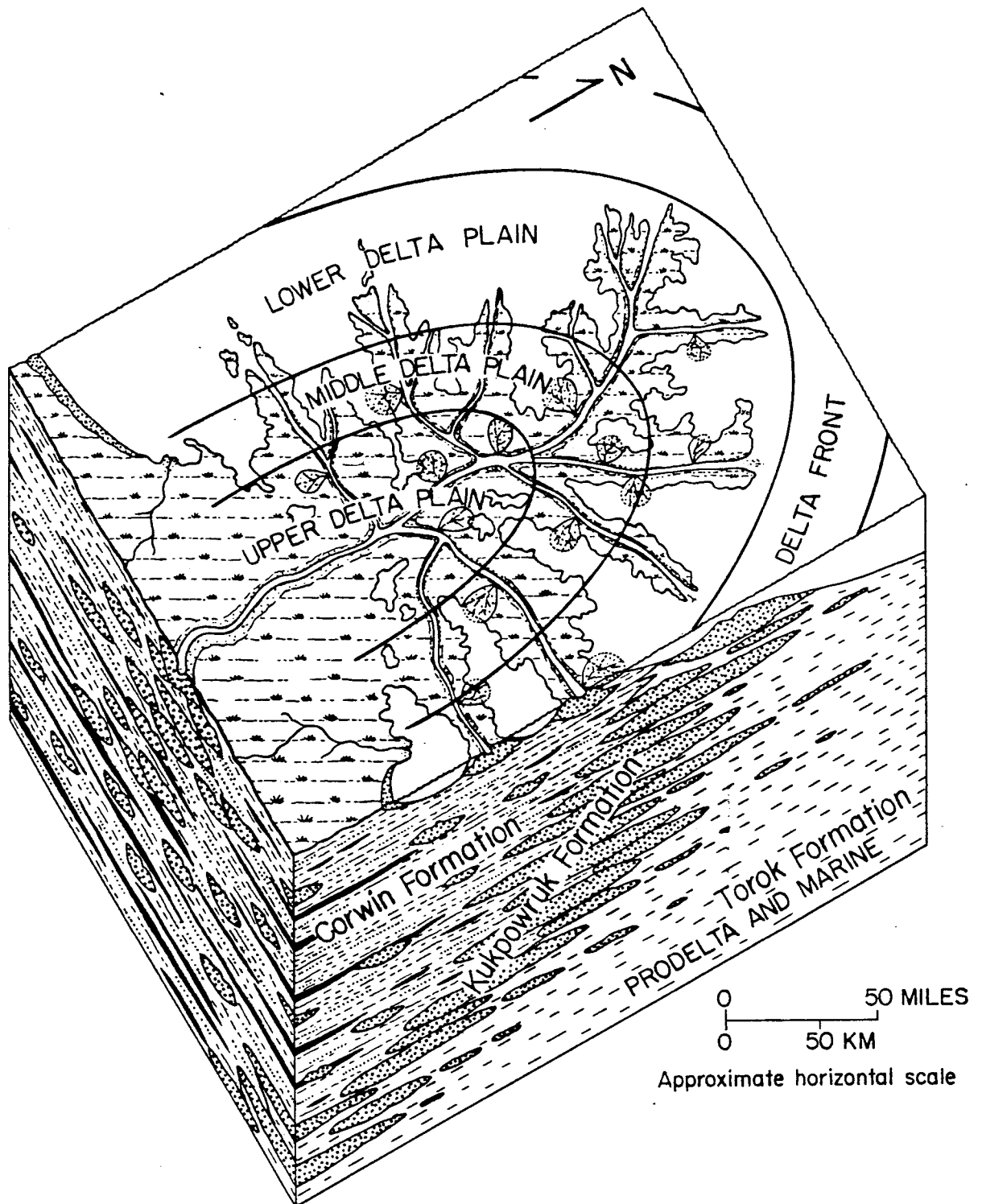
Fig. 5--Depositional environments of the Torok, Kukpowruk and Corwin Formations in northwestern Alaska. Lithologic symbols are identified on plate 2.
