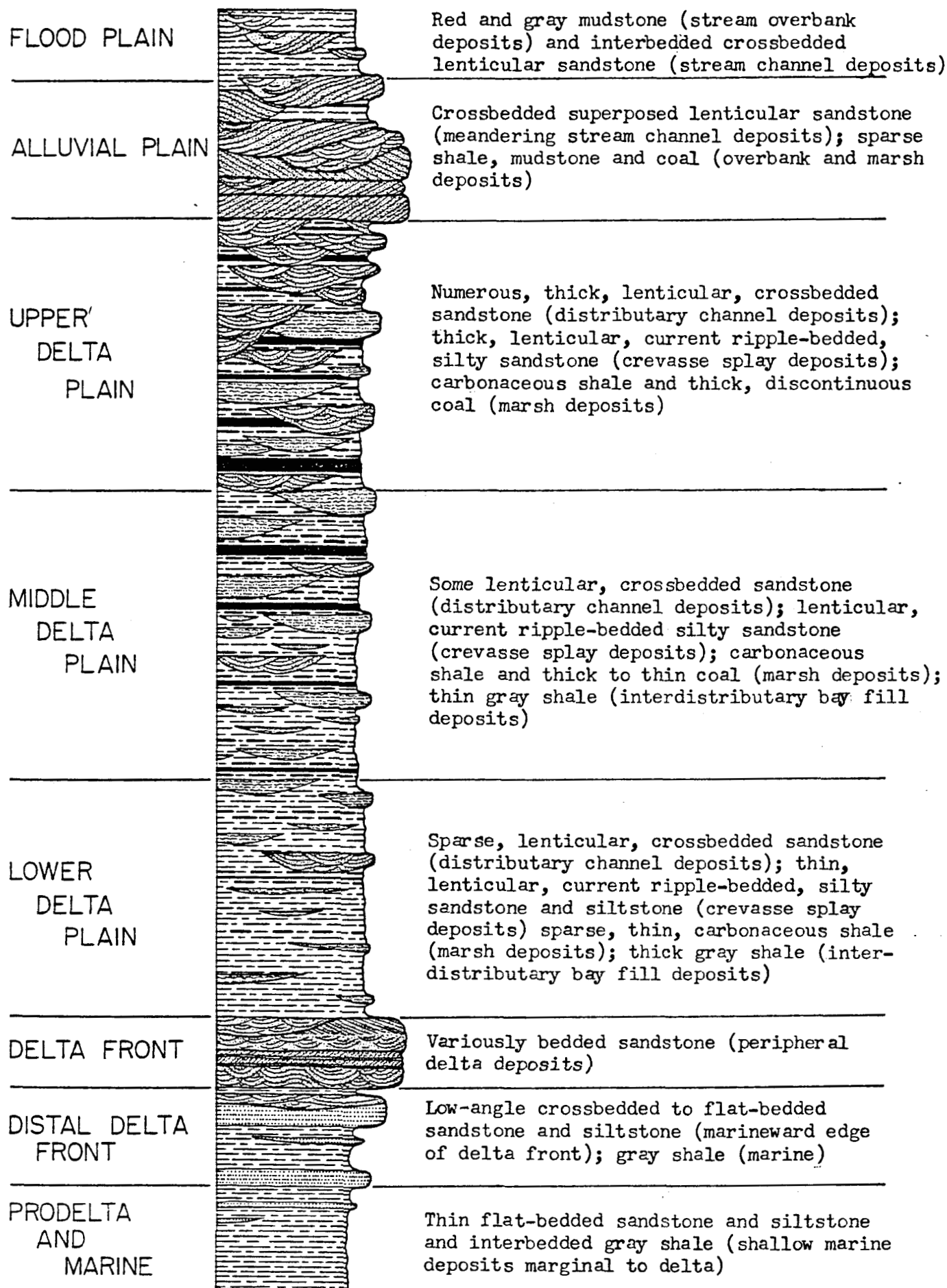
Fig. 4--Model of characteristic depositional environments and lithofacies of deltas and associated rocks in vertical succession.
