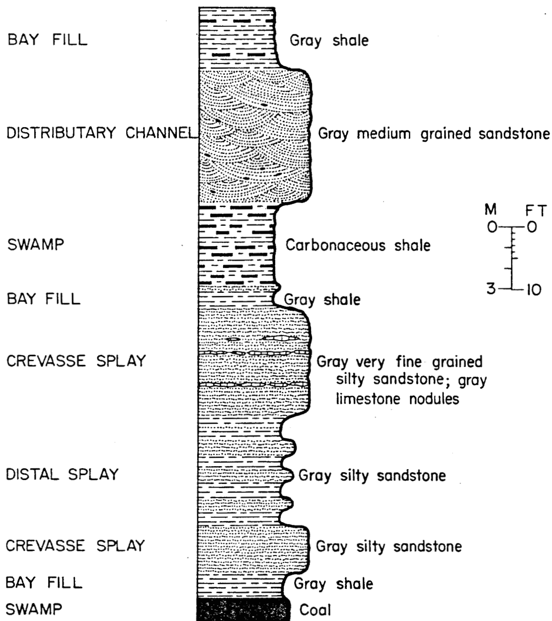
Fig. 12--Middle delta plain deposits in the Corwin Formation in WC sec. 24, T. 1 S., R. 36 W. (Section A478, beds 63-72).
