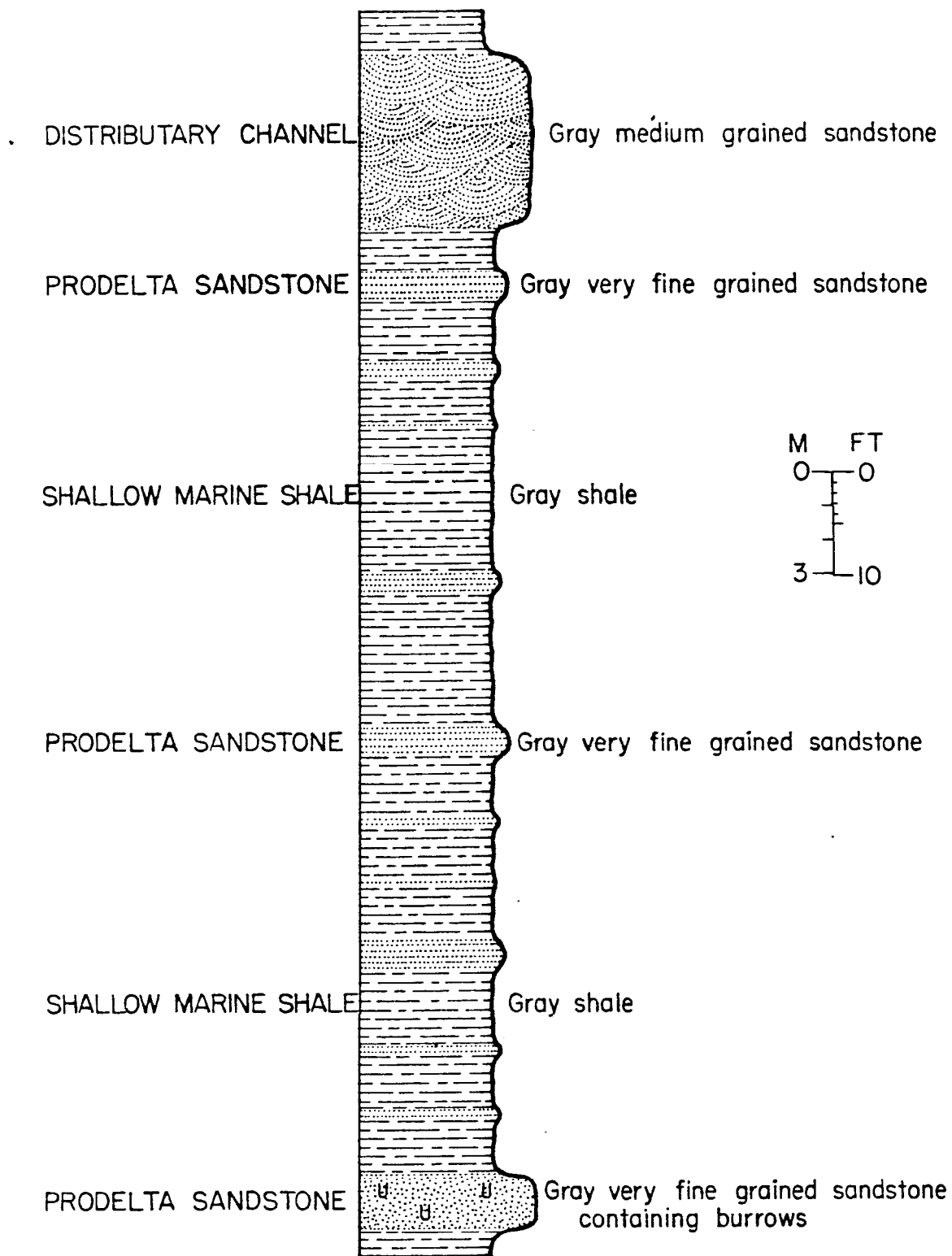
Fig. 6--Delta front deposits in the Kukpowruk Formation in NE \frac{1}{4} sec. 23, T. 1 S., R. 39 W. (Section A378, beds 10-13).
