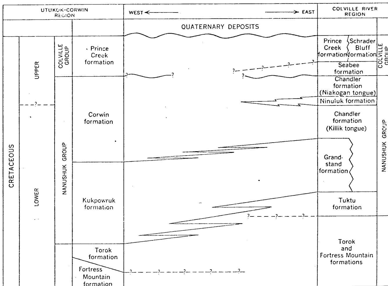
Fig. 2--West-east correlation of Cretaceous rocks in the National Petroleum Reserve in Alaska.
