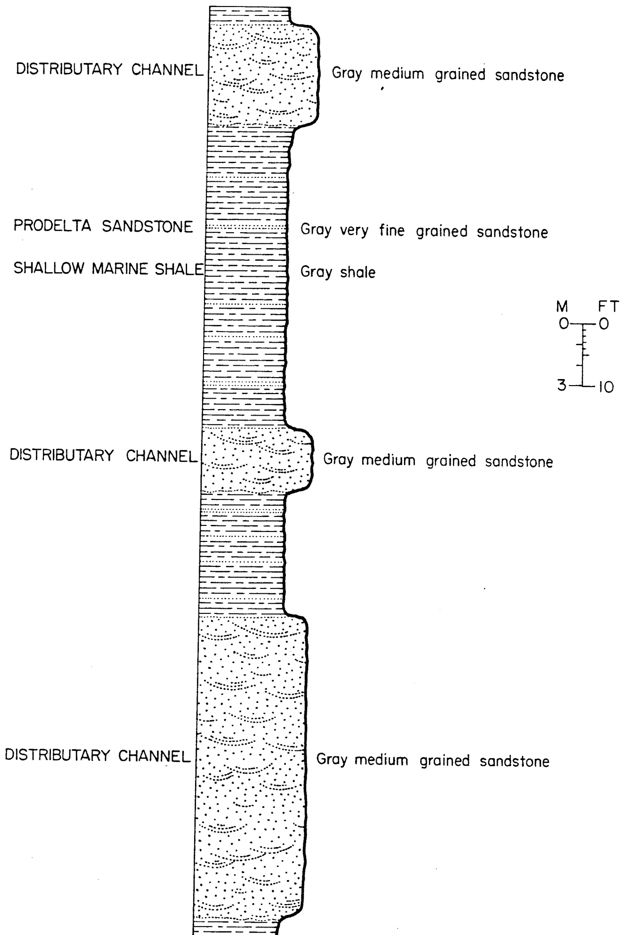
Fig. 7--Delta front deposits in the Kukpowruk Formation in W\frac{1}{2}NW\frac{1}{4} sec. 1 T. 2 S., R. 36 W. (Section A478, beds 18-23).
