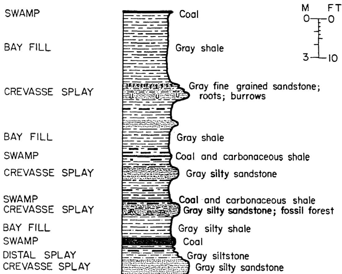
Fig. 13--Middle delta plain deposits in the Corwin Formation in SE\frac{1}{4}NE\frac{1}{4} sec. 2, T. 1 S., R. 39 W. (Section A378, beds 111-124).
