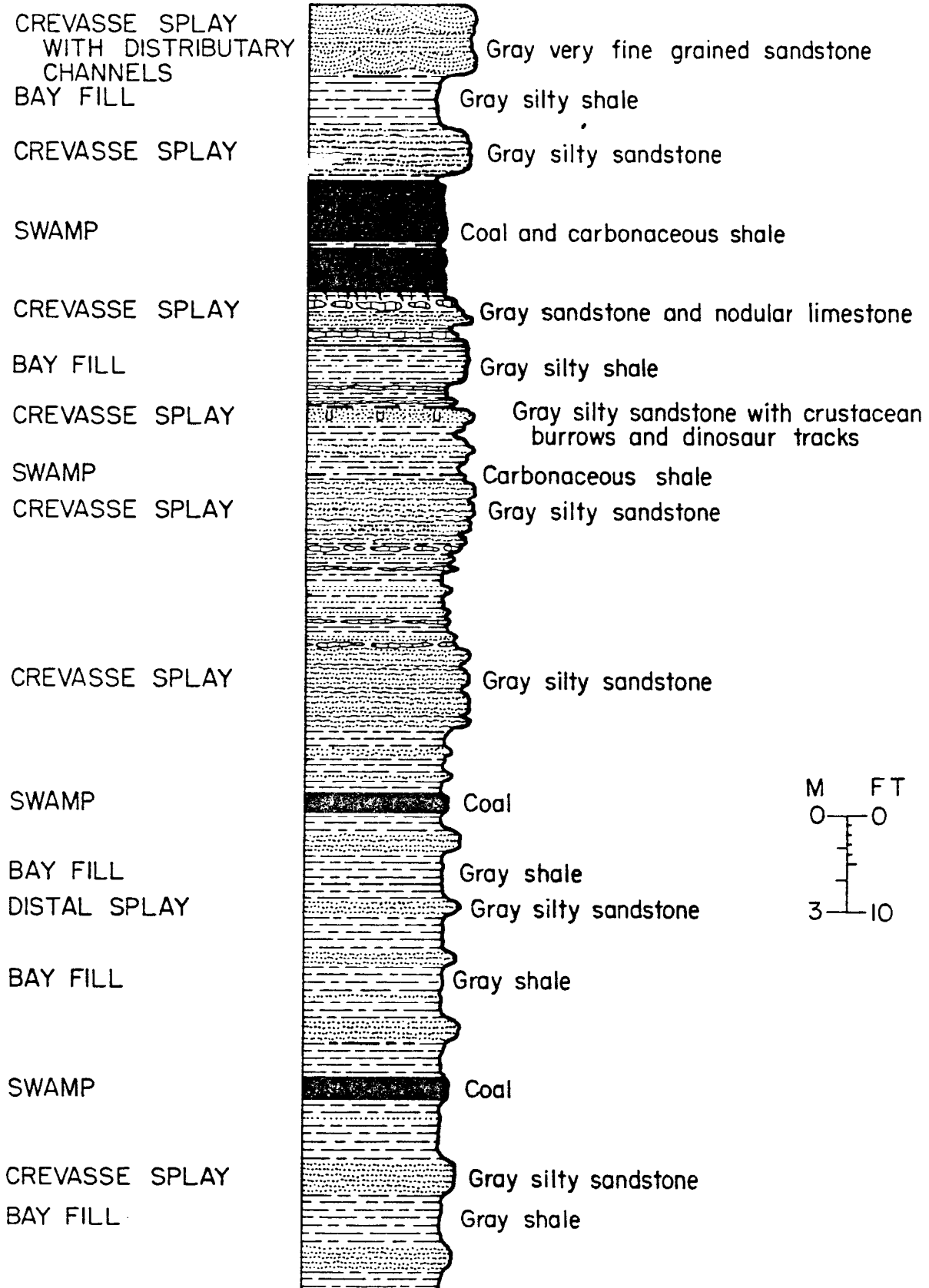
Fig. 11--Middle delta plain deposits in the Corwin Formation in NE \frac{1}{4} NW \frac{1}{4} sec. 13, T. 1 S., R. 40 W. (Section A278, beds 16-45).
