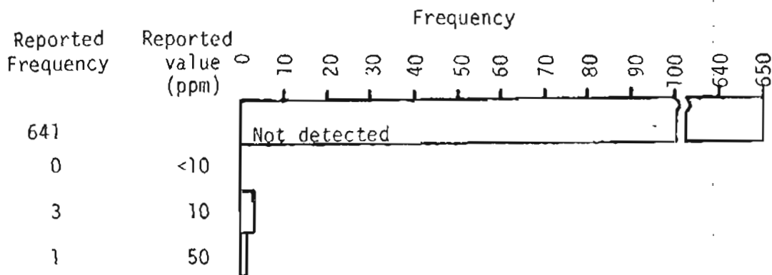
Figure 12.--Histogram showing molybdenum, in parts per million (ppm), in samples of the ash of black spruce needles from the Tanacross quadrangle, Alaska.
