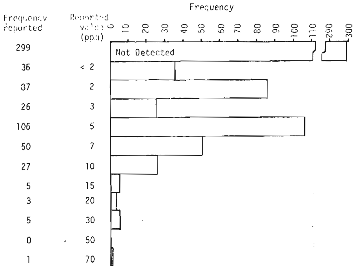
Figure 12.--Histogram showing molybdenum, in parts per million (ppm), in samples of the ash of black spruce needles from the Tanacross quadrangle, Alaska.
