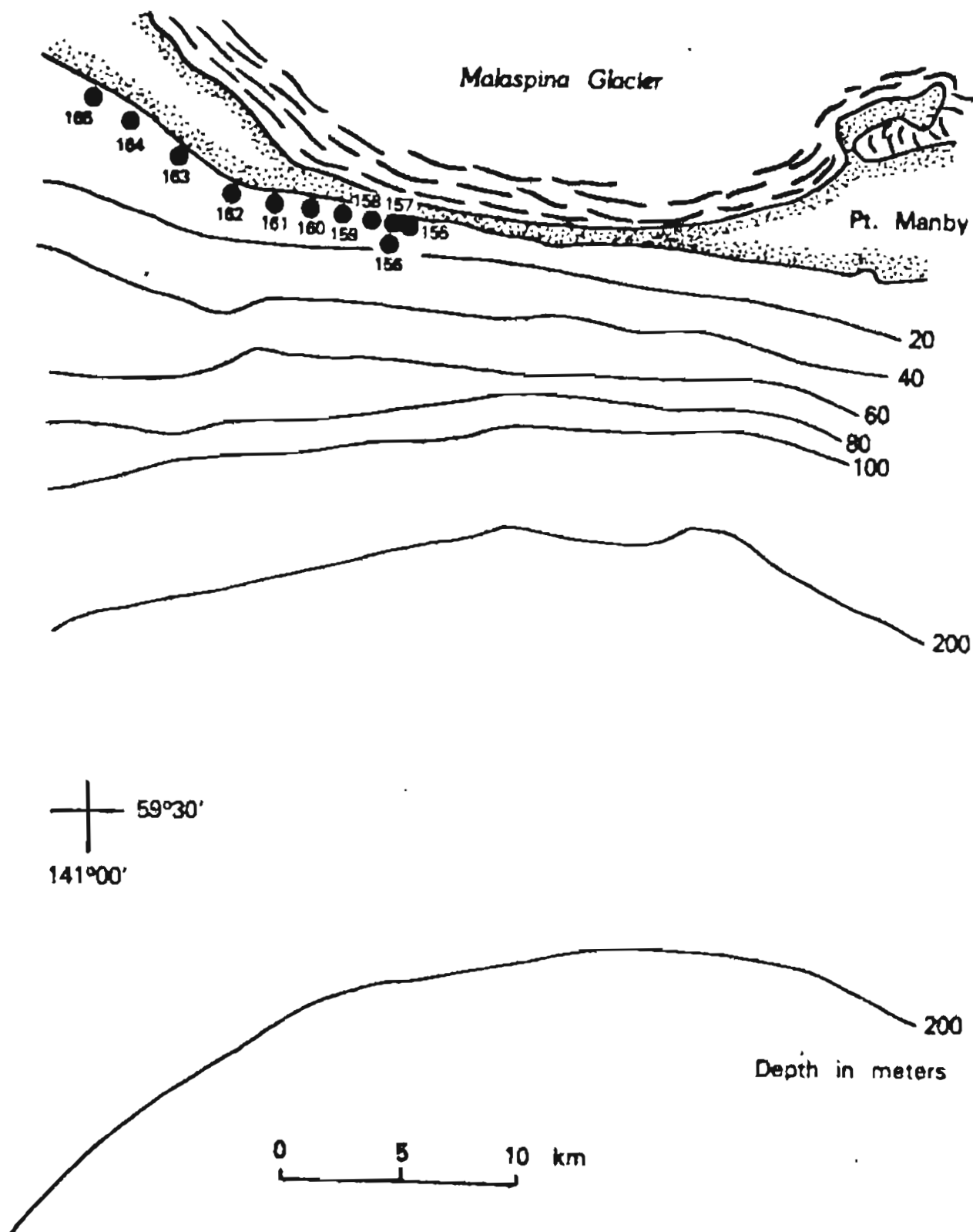
Figure 3.--Locality map showing samples collected between Icy Bay and Point Manby, from latitude 59^{\circ}45' \text{ N.} to 59^{\circ}15' \text{ N.} and longitude 140^{\circ}30' \text{ W.} to 141^{\circ}00' \text{ W.}
