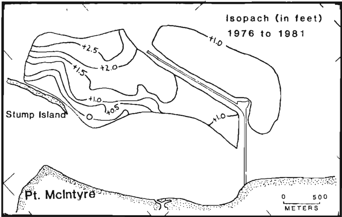
Figure 7. Isopach map (in feet) showing bathymetric changes from 1976 to 1981. Area isopached is same as figure 6.
