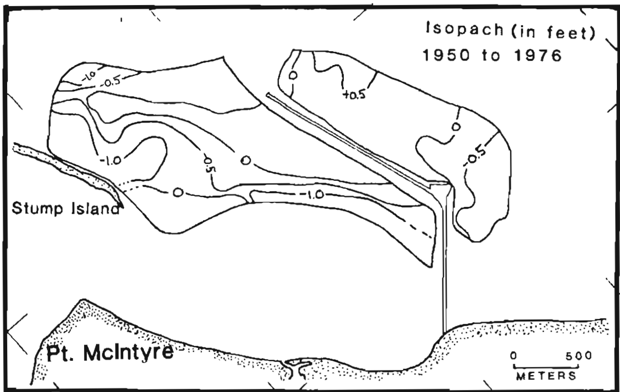
Figure 6. Isopach map (in feet) showing bathymetric changes from 1950 to 1976. Positive values indicate depth decreases (deposition) and negative values indicate depth increases (erosion). Limit of isopach map is determined by the limit of overlapping data 1950 and 1976. (See Figs. 3 and 4).
