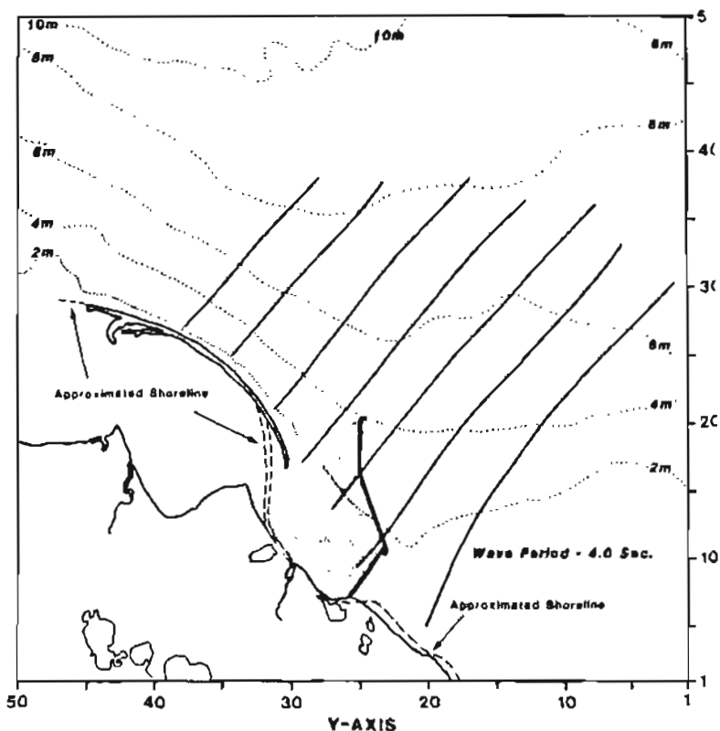
Figure 11. Wave orthogonals from northeast wind with suggested areas of reduced wave energy in the quiet "backwater" of West Dock (from Harper, 1982). Bathymetry is pre-causeway construction.
