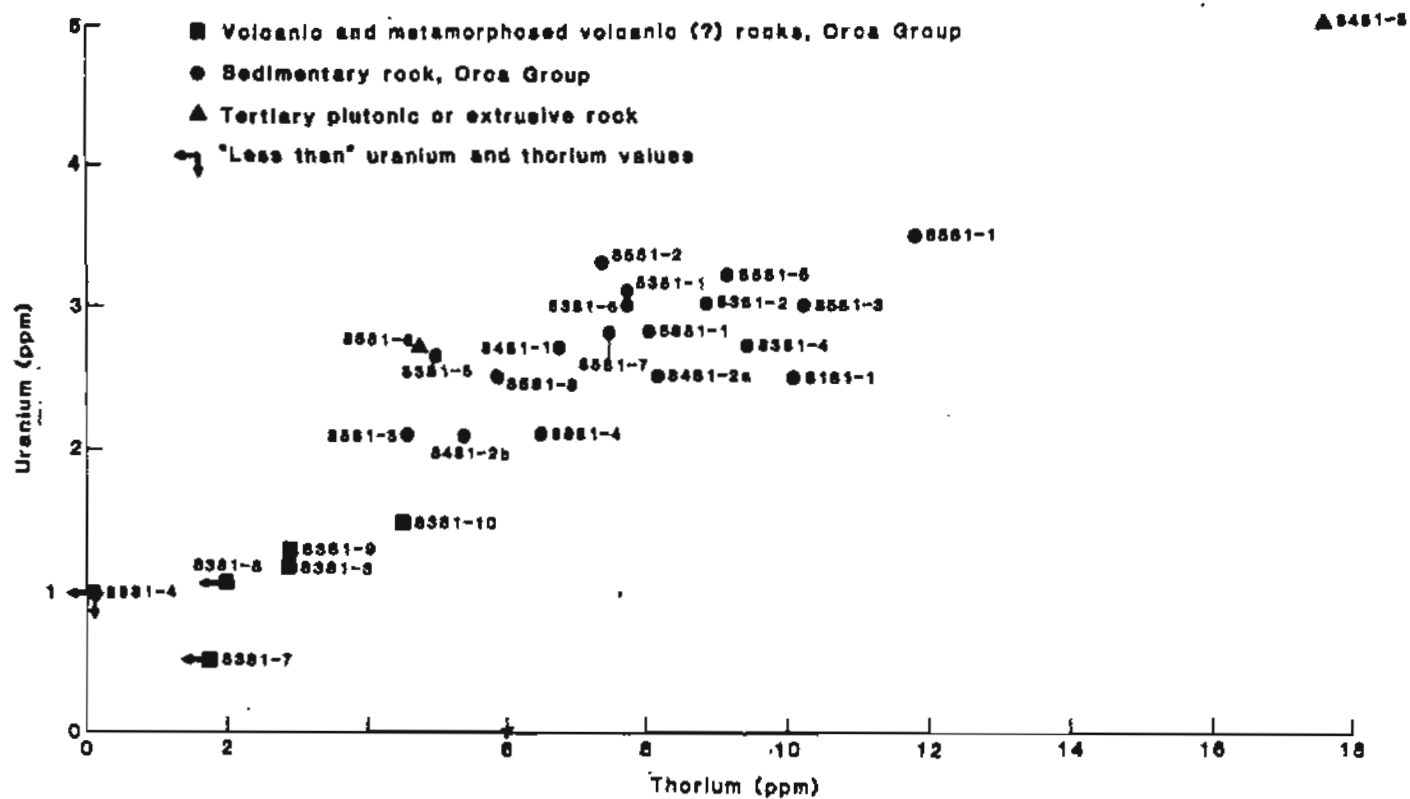
Figure 2.--Graph of uranium versus thorium from samples of the Orca Group and related plutonic rocks.
