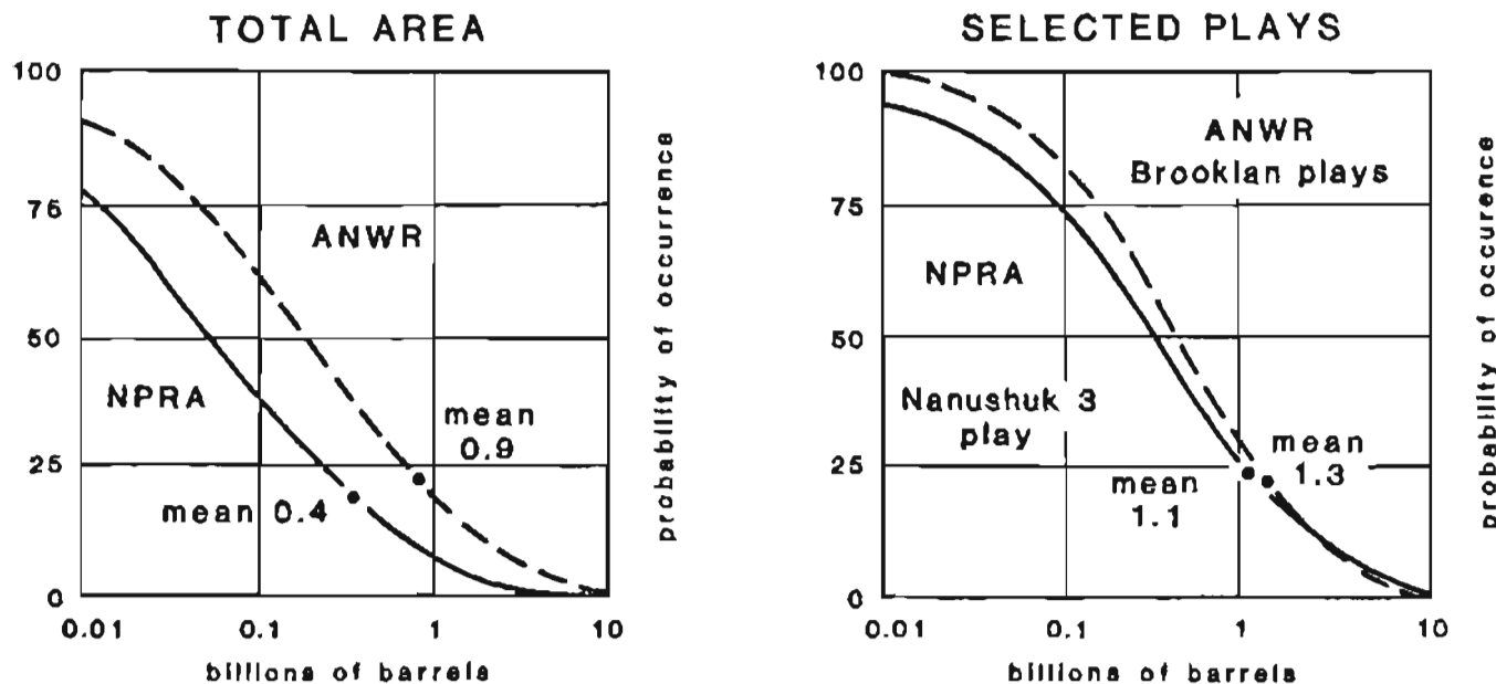
Figure 6. A comparison of probability distributions of undiscovered oil and gas resources and pool sizes for the NPRA (solid curve) and the ANWR (dashed curve). The larger ANWR pool sizes compared to the NPRA pool sizes (lower left diagram) are the result of very large pool sizes in ANWR Brookian plays. These plays are geologically most similar to the NPRA Brookian Nanushuk 3 play (number 5 on Fig. 4) and comparison shows they have similar pool sizes (lower right diagram).
