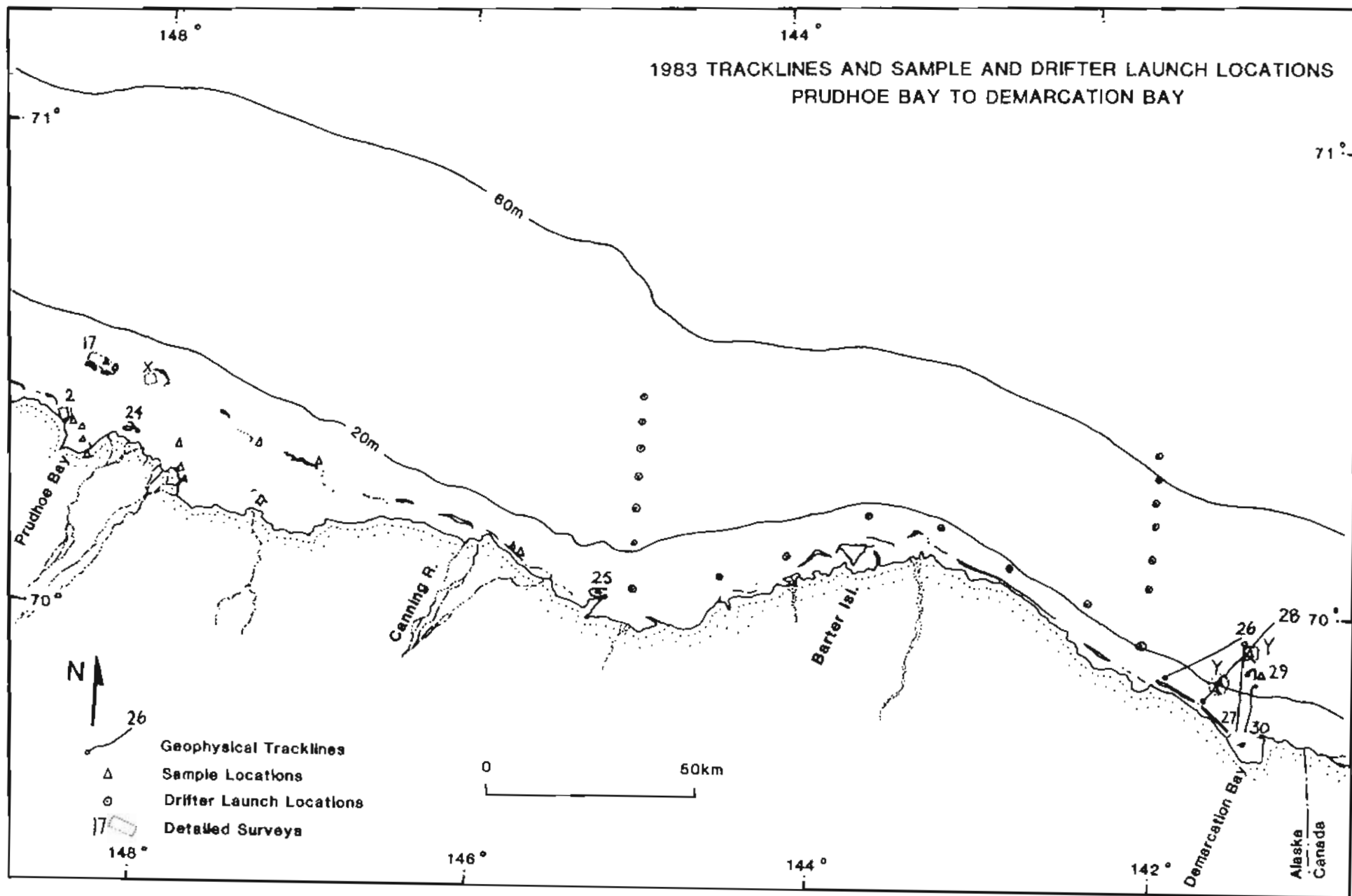
Figure 1. 1983 geophysical tracklines, and drifter launch and sample locations between Demarcation Bay and Prudhoe Bay. Line and location numbers are those used in tables 1, 2, and 3.
