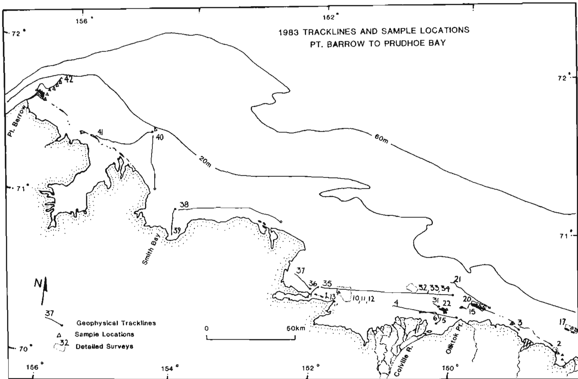
Figure 2. 1983 geophysical tracklines and sample locations between Prudhoe Bay and Point Barrow.
