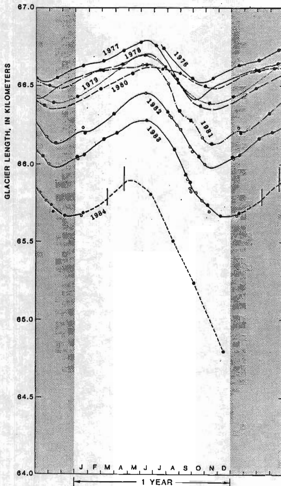
Figure 3.--Seasonal advance and retreat of Columbia Glacier for the years 1976-84, superimposed onto one year for comparison. The curves are repeated in the gray areas to either side to help visualize trends. Solid dots are data points obtained by photogrammetry (error is about 10 m), open circles are observations by less-accurate methods (ship-borne radar, ground surveys), and smooth curves are drawn through data points. Data from aerial photographs taken on March 12 and April 24, 1984, are plotted as vertical lines because of the difficulty in differentiating the low, irregular ice cliff from floating ice. Values are averaged over the width of the active terminus.
