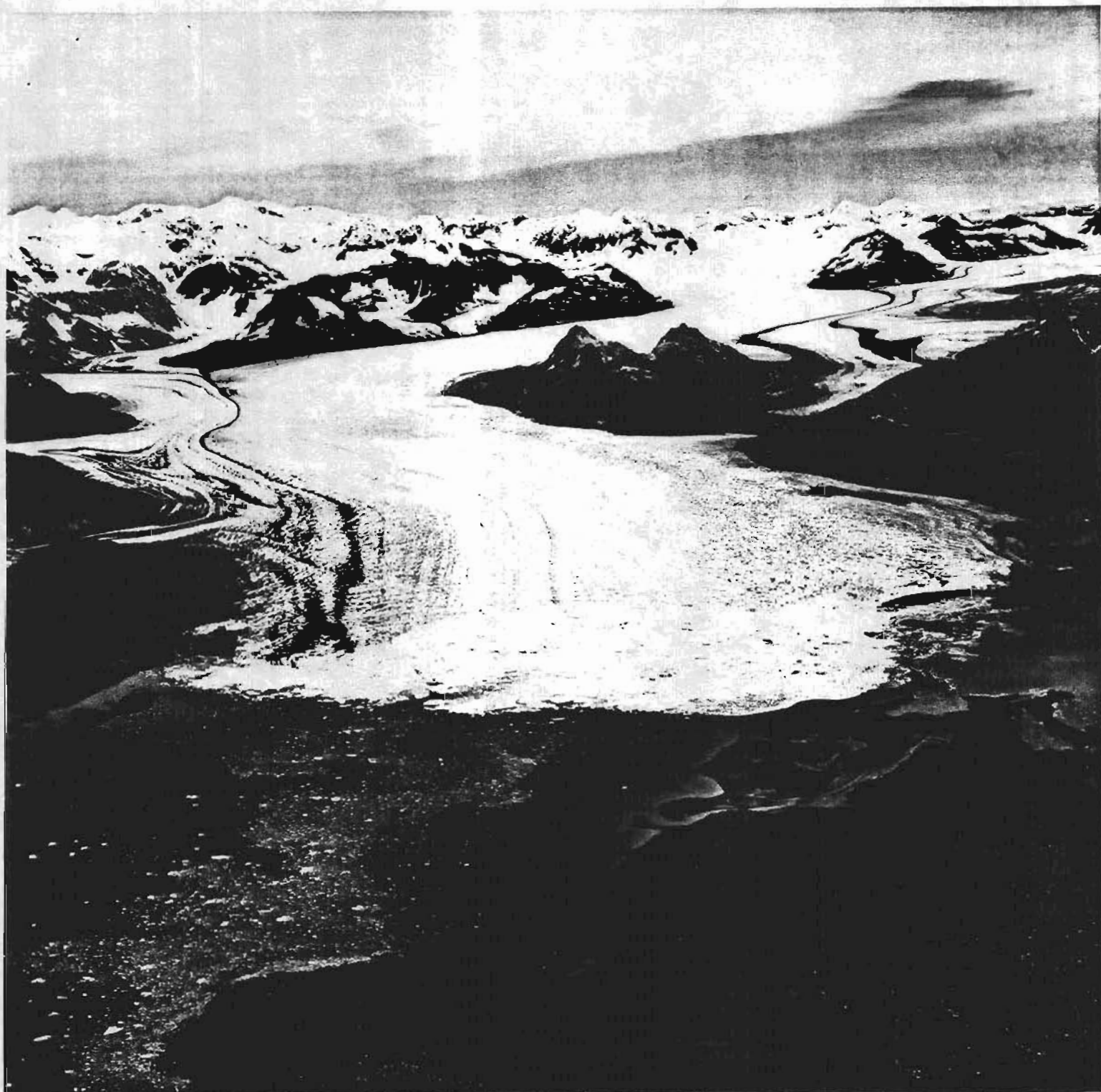
Figure 1.--Oblique aerial photograph of the lower Columbia Glacier. View is to the north, and Heather Island is in the foreground. The ice cliff is about 30 to 70 m high and makes up 5 km of the width of the terminus. The position of a terminal moraine shoal, connecting Heather Island with both sides of the fiord, can be inferred from the lines of stranded icebergs that block the movement of other pieces of ice, causing much of the water surface near the terminus to be covered with ice. The point of ice near the west (left) side of the terminus (marked with streaks of debris) disappeared completely by December 14, 1984. USGS photograph by Robert M. Krimmel, August 29, 1984.
