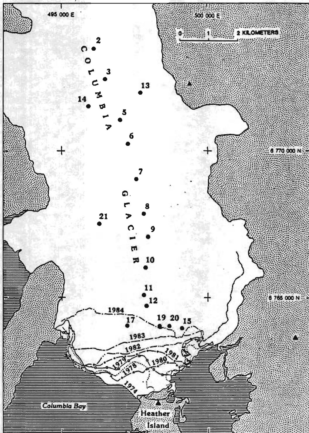
Figure 4.--Map showing the configuration of the terminus of Columbia Glacier after summer retreat, for the years 1974 and 1978-84. Small crosses represent the Universal Transverse Mercator coordinates in meters. Also indicated are the marker locations (dots) and survey stations (triangles) used during the August, 1984 field program. Markers numbers 2, 3, 5-11 and 17 are on or near the main stream of the glacier flow. Marker 17 was on the glacier in August but the terminus subsequently retreated back from that location.
