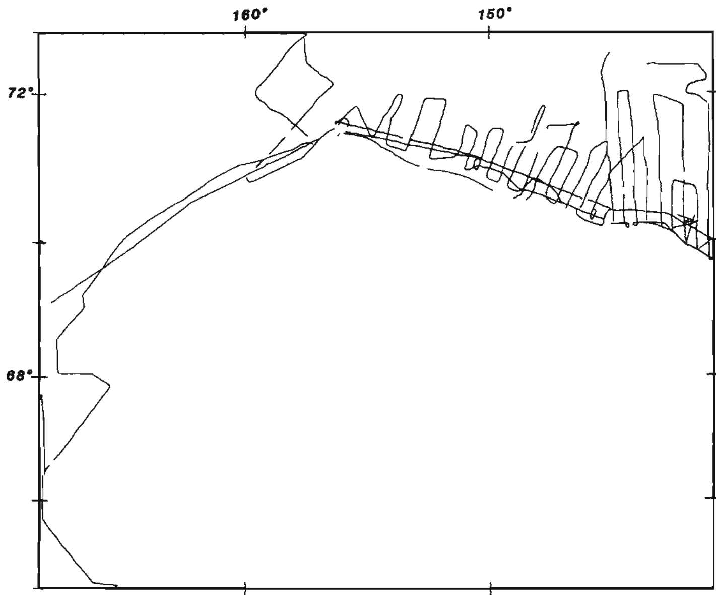
Figure 2.--Location of U.S. Geological Survey R/V S. P. LEE cruise L977AR digital marine gravity data collected in the Beaufort Sea and eastern Chukchi Sea in 1977.
