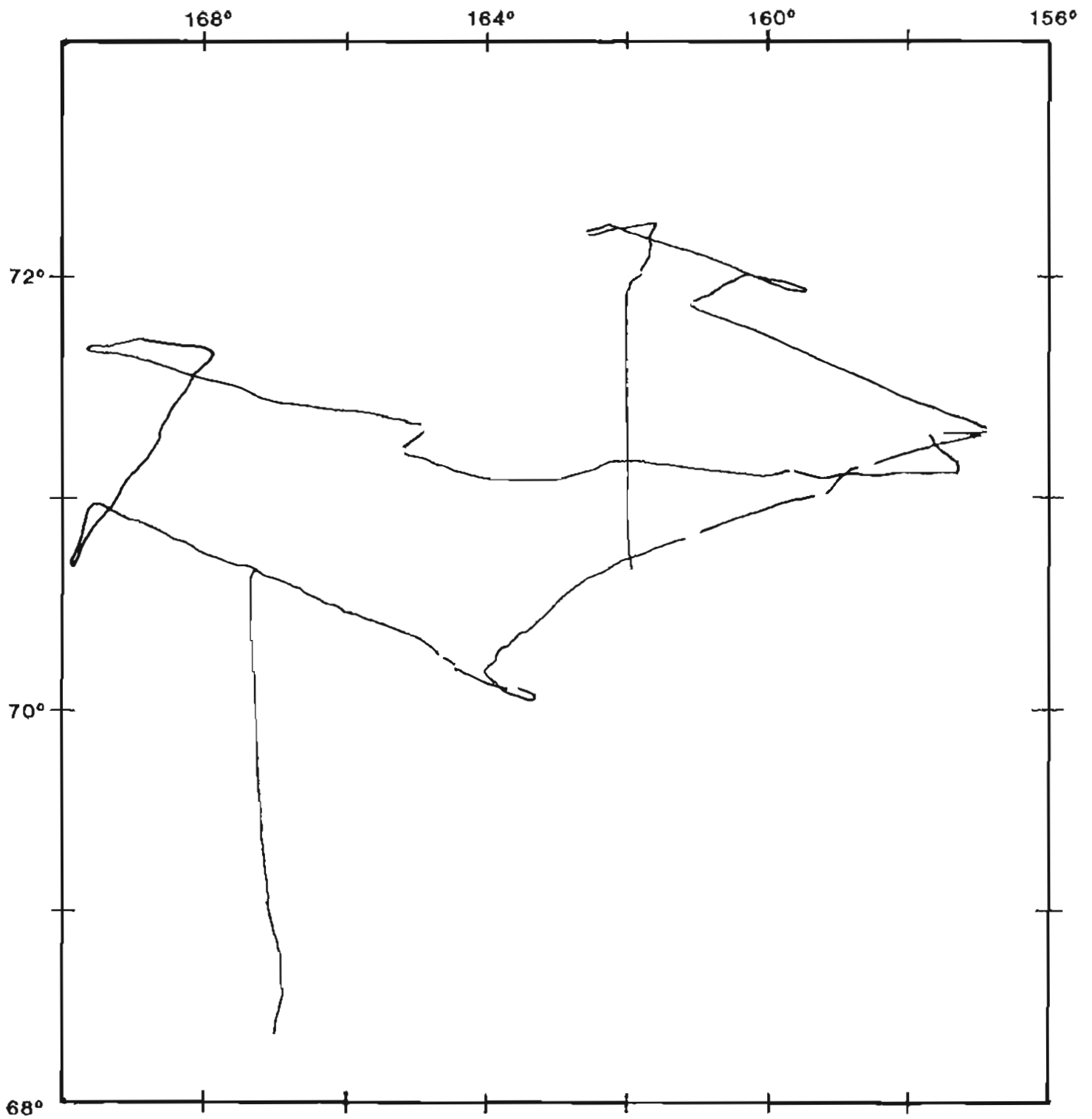
Figure 2.--Location of U.S. Geological Survey R/V S. P. LEE cruise L1182CS digital marine gravity data collected in the central Chukchi Sea in 1982.
