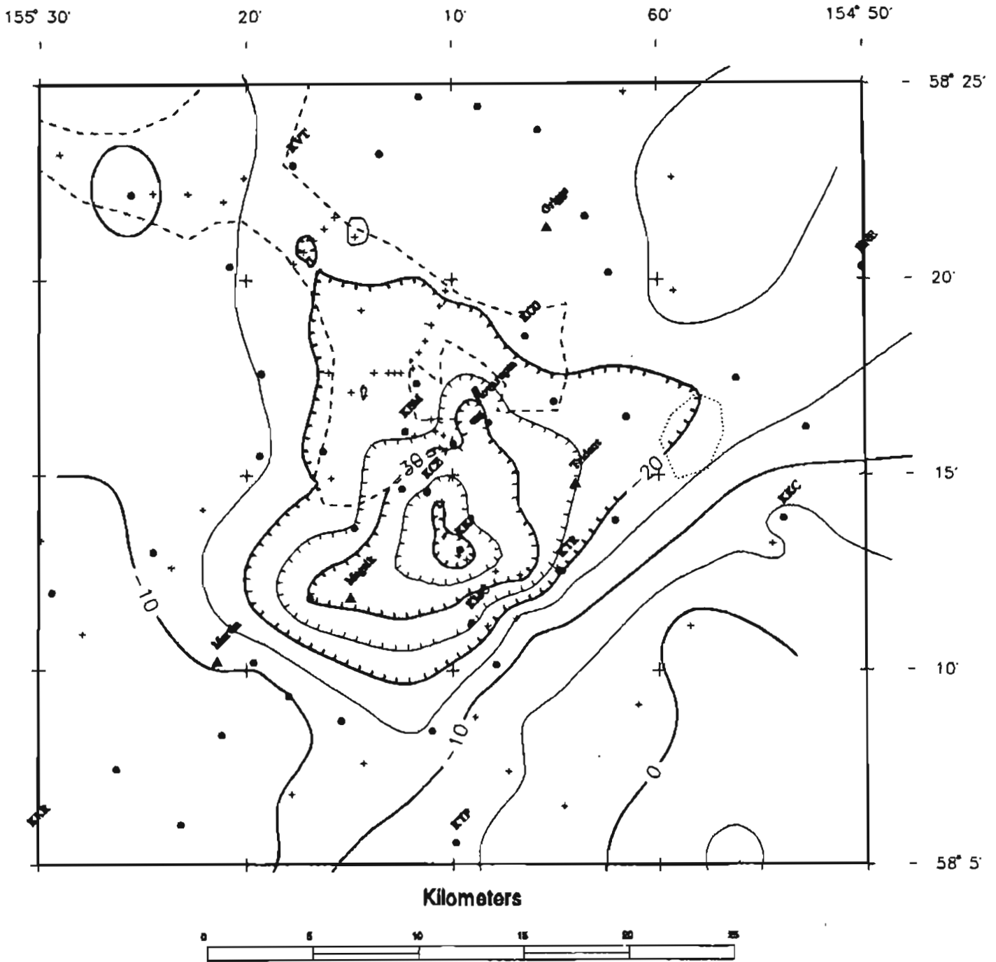
Figure 6: Complete Bouguer gravity anomaly in the vicinity of Katmai Pass, Katmai National Park, Alaska. Contour interval is 5 mGal. Dashed line traces the Valley of Ten Thousand Smokes, dotted line outlines Katmai Caldera. Triangles mark major volcanos. Filled circles are the locations of new gravity measurements from July 1991, pluses mark previous measurements (Keinle, 1969; David Barnes, written communication, 1990). Three-letter labels identify stations of the seismic network (Ward et al., 1991). Station KKP is located at Katmai Pass.
