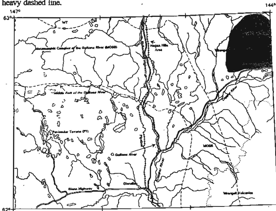
Figure 2. Generalized map showing geology and mining districts. Three bedrock terranes identified in the quadrangle are the Peninsular Terrane (PT), the Metamorphic Complex of Gulkana (MCGR), and the Wrangellia Terrane (WT). The quaternary volcanic rocks of the Wrangell Mountains overlie Wrangellia Terrane in the southeast corner of the quadrangle. The Ahtell Creek mineralized area is located in the northeast corner of the quadrangle and is shaded. The Hogan Hills mineralized area is located near the center of the quadrangle.
