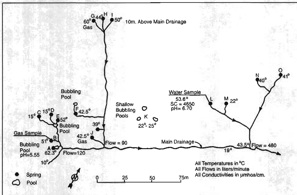
Figure 2. Detail at Cold Bay Hot Springs. From Motyka, and others (1981).
