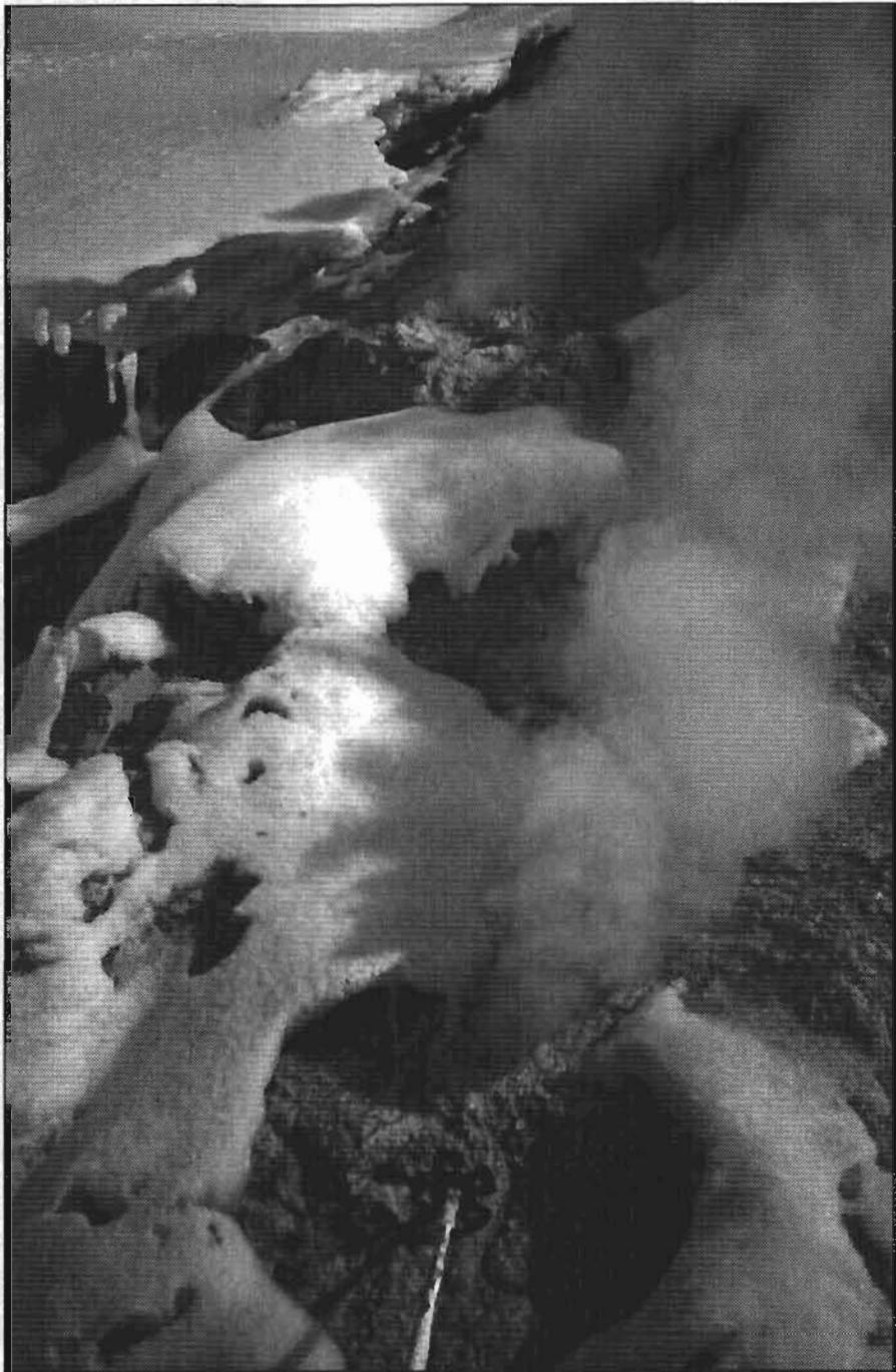
Figure 8. Fumaroles and sulfurous rocks on the east flank of Mt. Hague. Ski pole tip is in the photograph for scale. Photo taken April 6, 1996.
