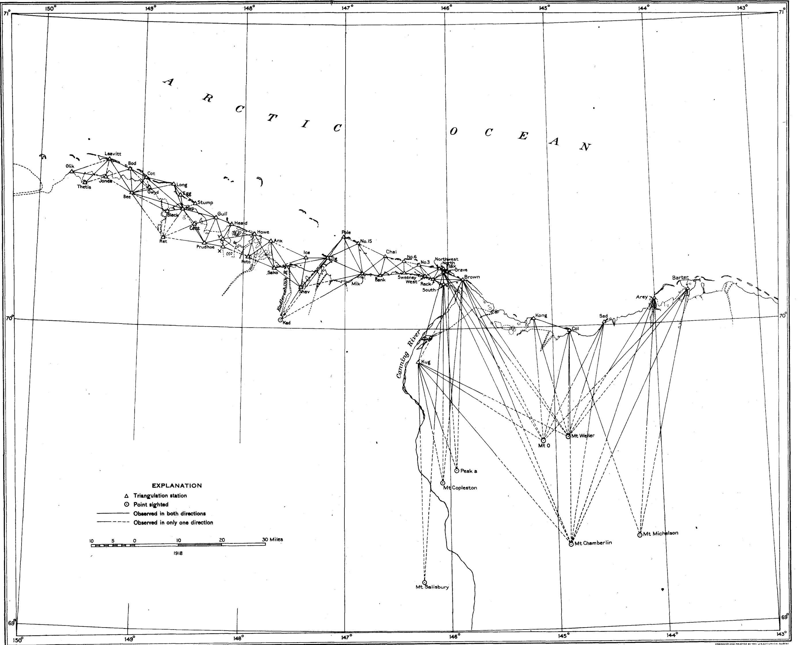
TRIANGULATION STATIONS ALONG THE ARCTIC COAST ADJACENT TO CANNING RIVER, ALASKA
