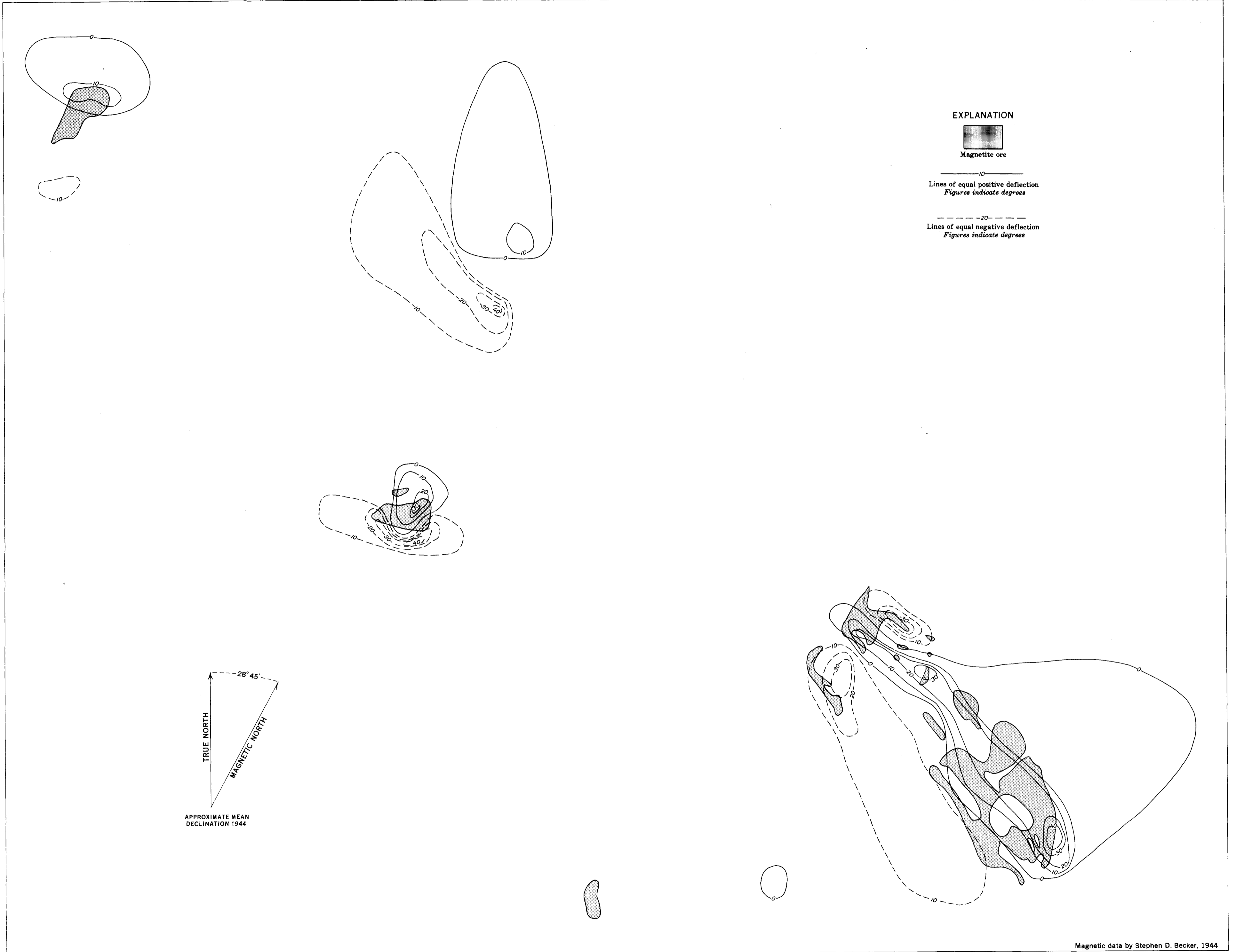
ISOMAGNETIC MAP OF UPPER MAGNETITE AREA, SHOWING LINES OF EQUAL DIP-NEEDLE DEFLECTION, JUMBO BASIN, PRINCE OF WALES ISLAND, SOUTHEASTERN ALASKA
