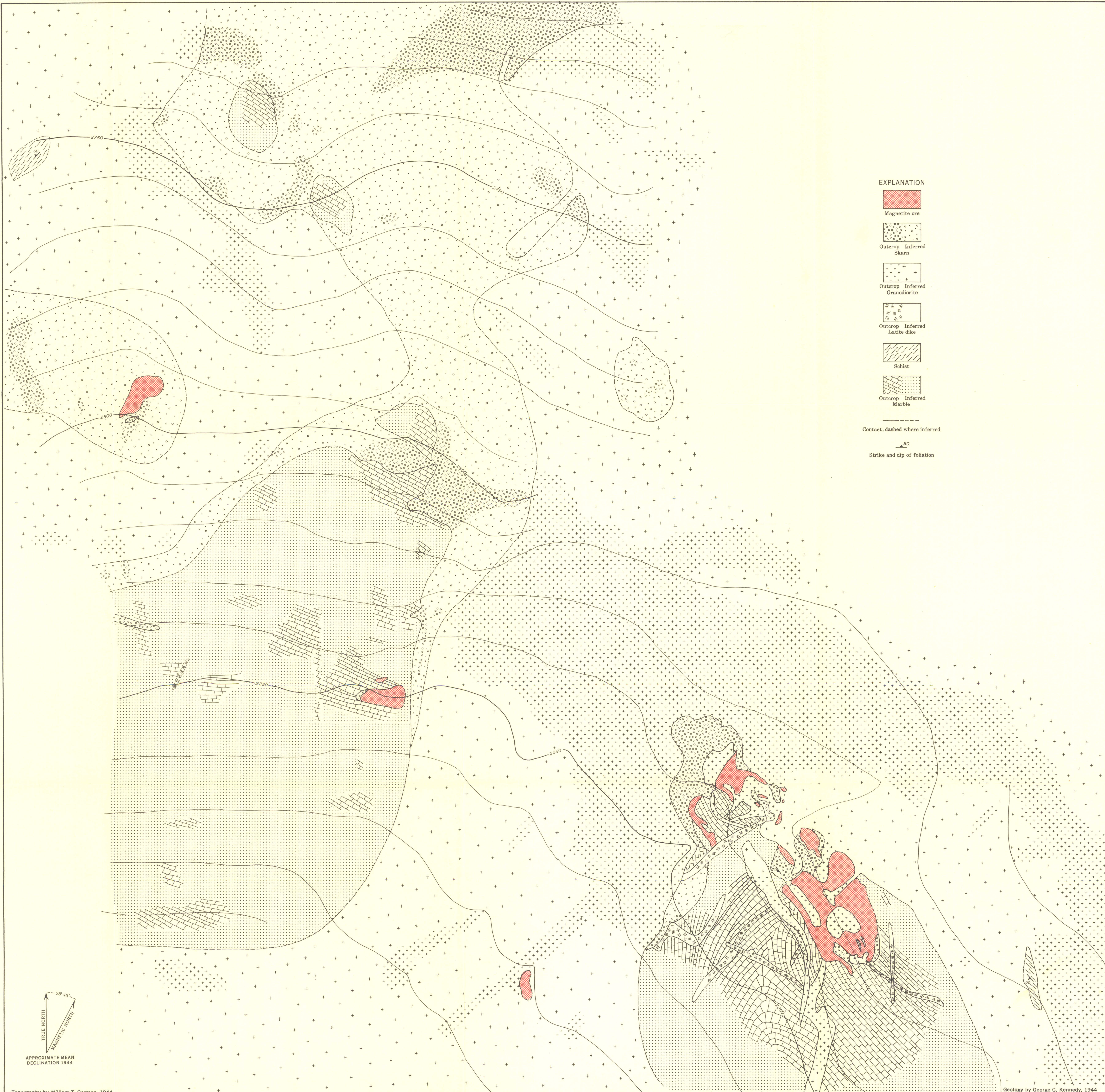
GEOLOGIC MAP OF UPPER MAGNETITE BODIES AND VICINITY, JUMBO BASIN, PRINCE OF WALES ISLAND, SOUTHEASTERN ALASKA
