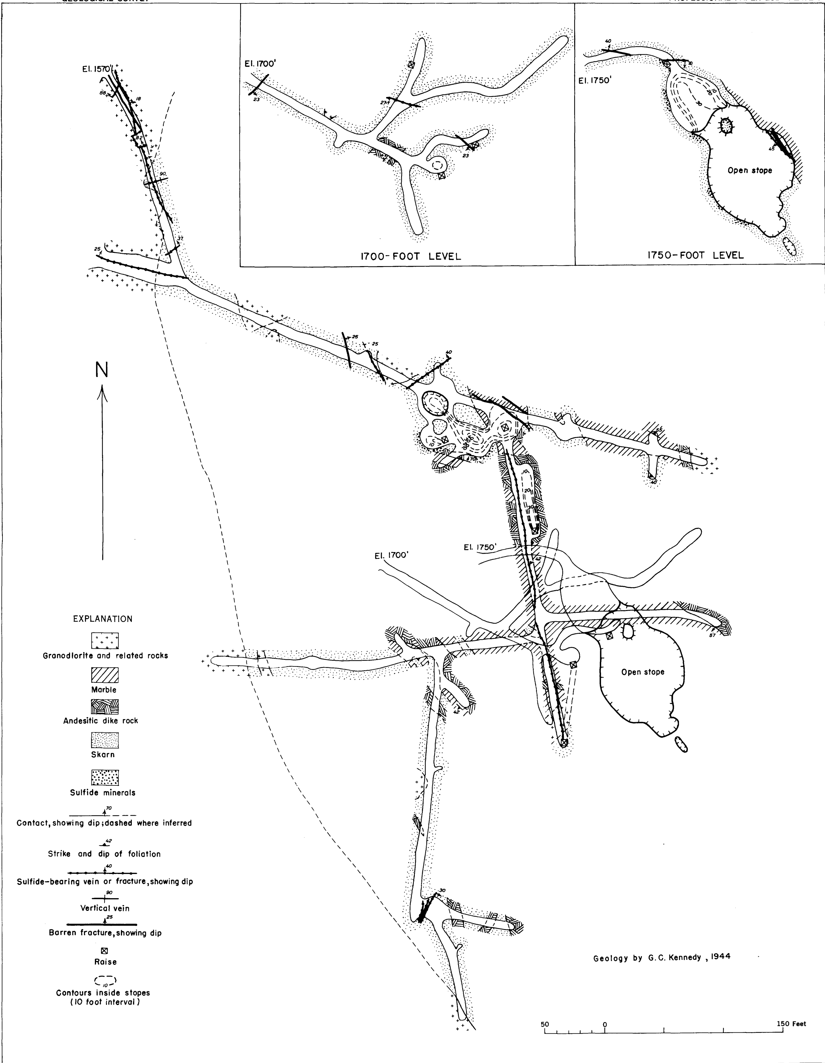
GEOLOGIC MAP OF THE JUMBO MINE, JUMBO BASIN, PRINCE OF WALES ISLAND, SOUTHEASTERN ALASKA
