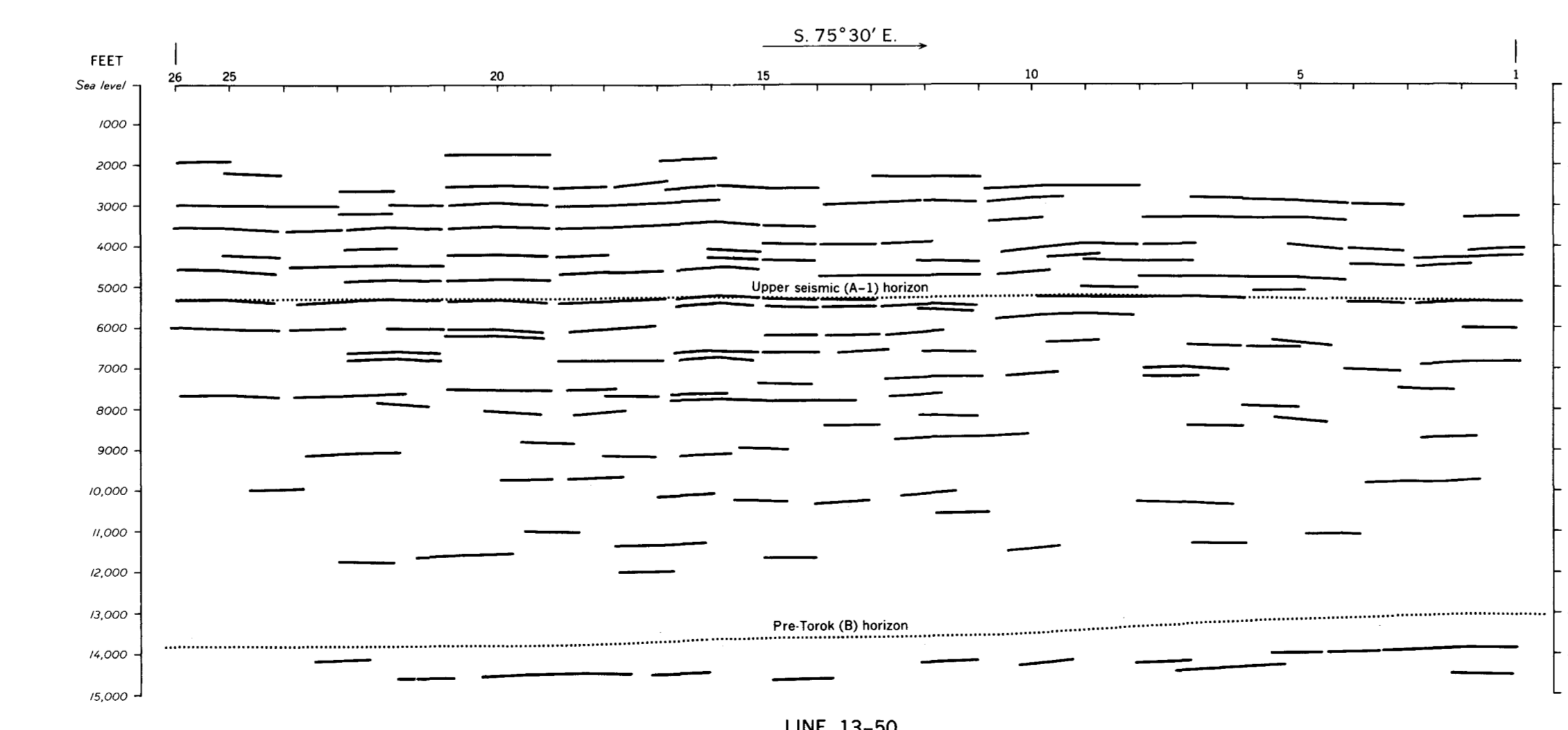
SEISMIC REFLECTION PROFILES, UPPER KAOLAK RIVER AREA, UTUKOK-CORWIN REGION, ALASKA Scale 1:62 500 0 1 2 3 4 5 Miles
