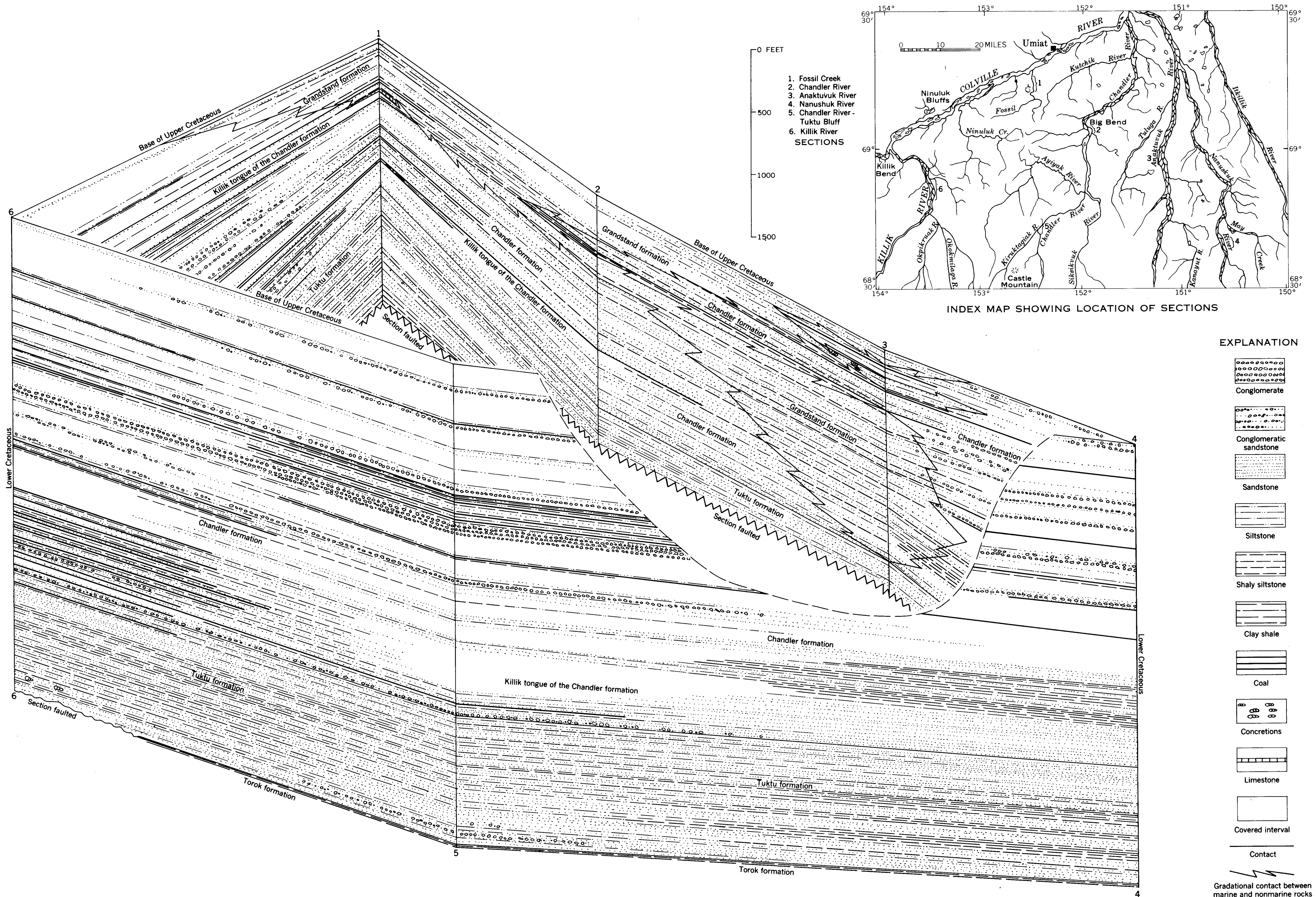
FENCE DIAGRAM OF THE TUKTU, CHANDLER, AND GRANDSTAND FORMATIONS
