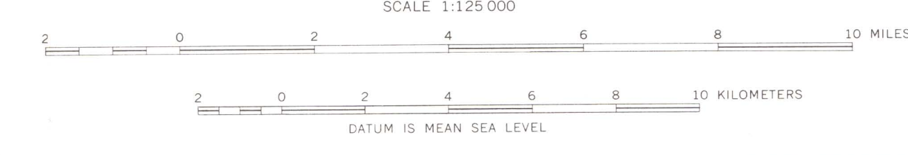
RECONNAISSANCE GEOLOGIC MAP AND GENERALIZED SECTIONS OF THE KILLIK-ITKILLIK REGION, ALASKA
