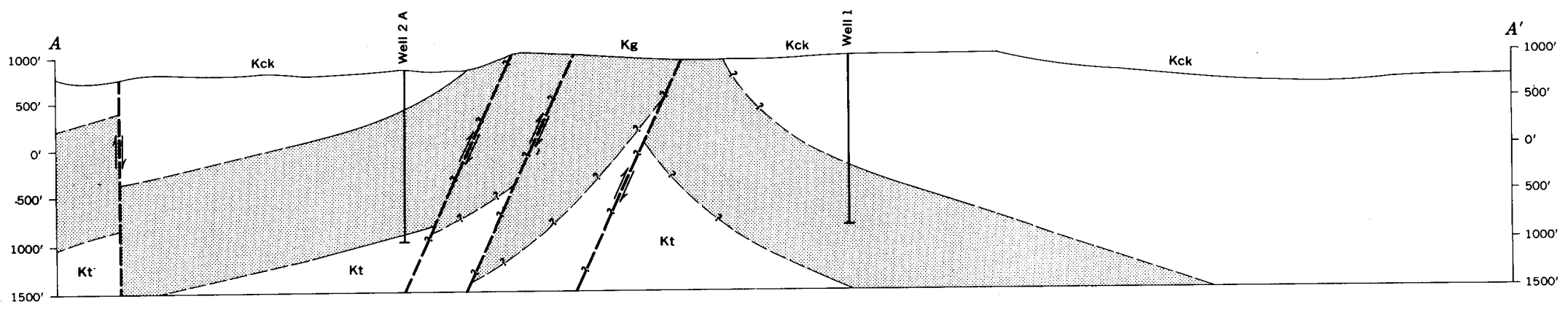
GEOLOGIC SKETCH MAP AND SECTION OF THE KNIFEBLADE ANTICLINE IN THE VICINITY OF THE KNIFEBLADE TEST WELLS, ALASKA
