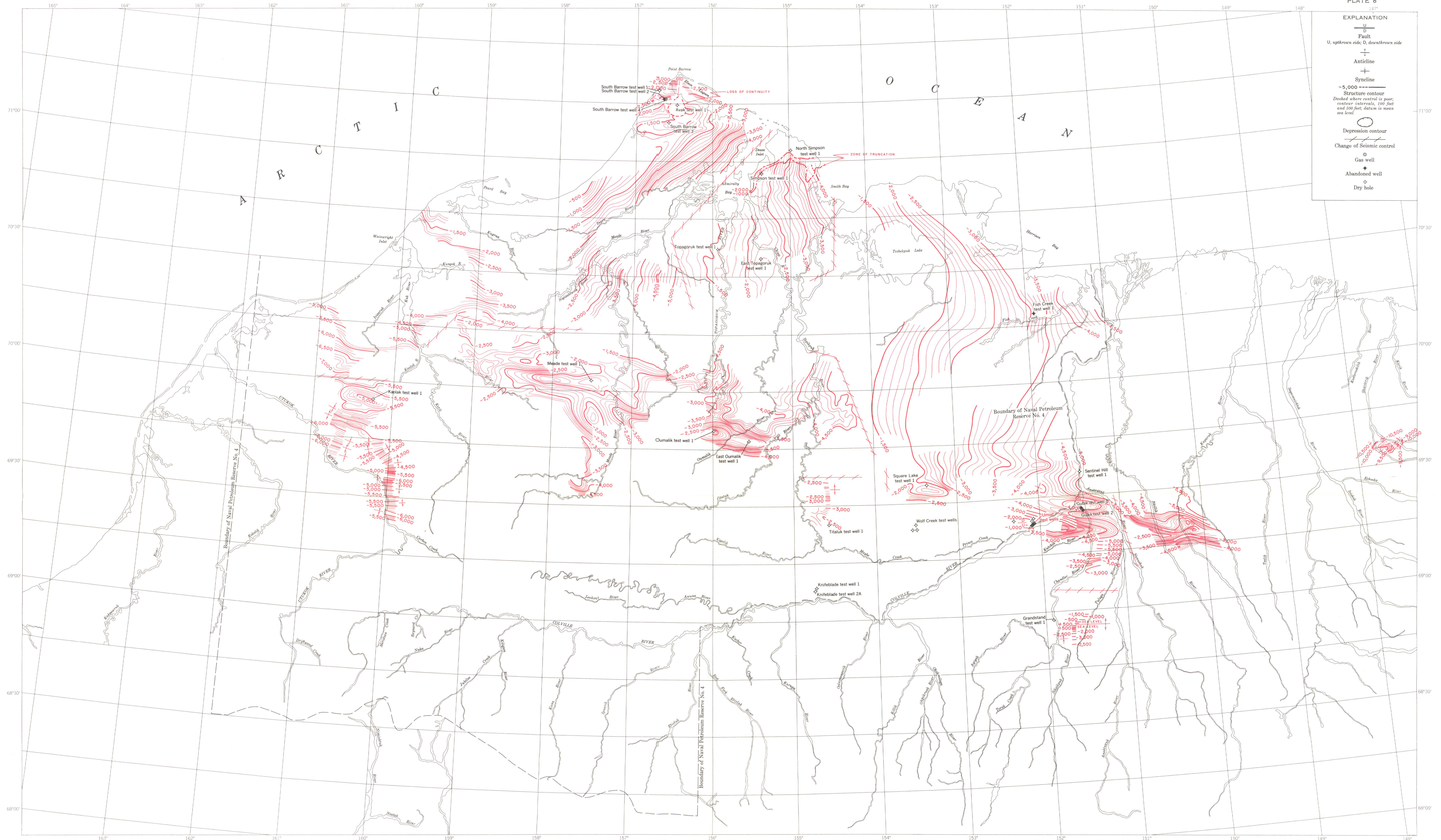
STRUCTURE-CONTOUR MAP OF NORTHERN ALASKA, CONTOURED ON A SEISMIC HORIZON IN SHALLOW CRETACEOUS ROCKS
