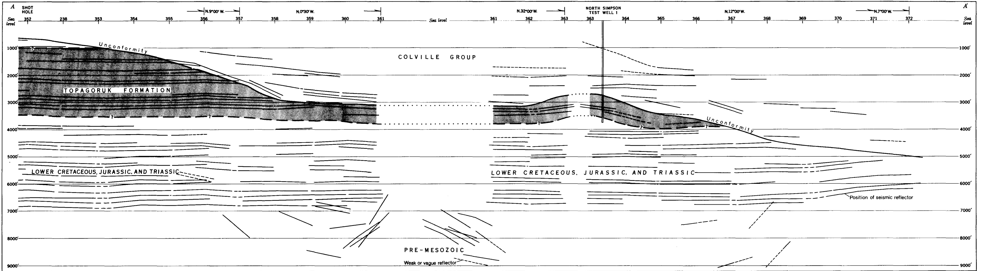
PART OF SEISMIC PROFILE (LINE 10-46) THROUGH NORTH SIMPSON TEST WELL 1, SIMPSON AREA, ALASKA
