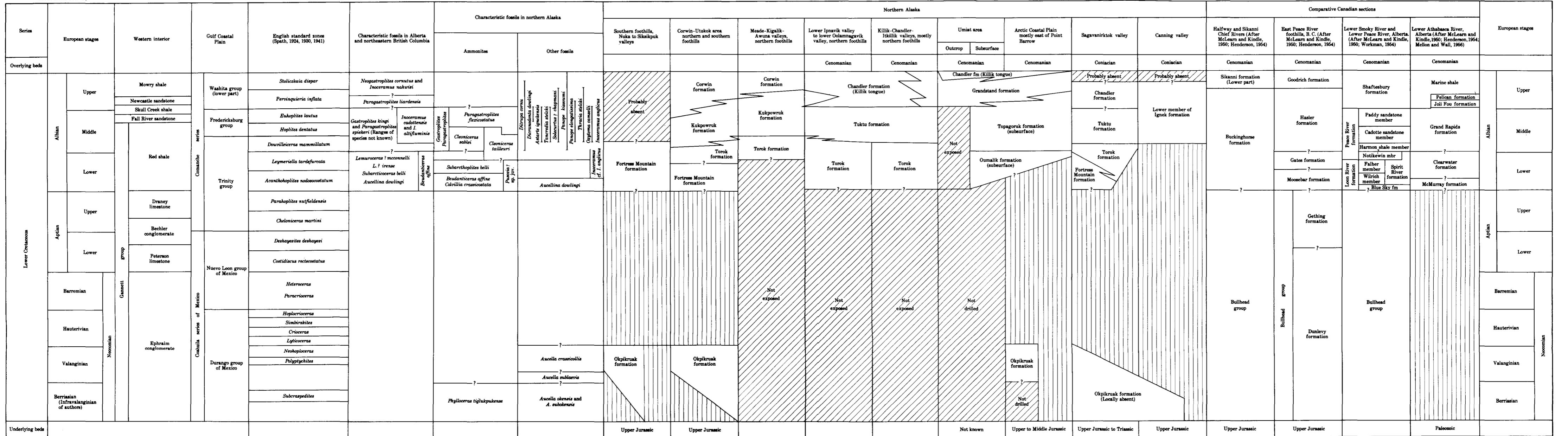
CORRELATION OF THE LOWER CRETACEOUS FORMATIONS IN NORTHERN ALASKA
