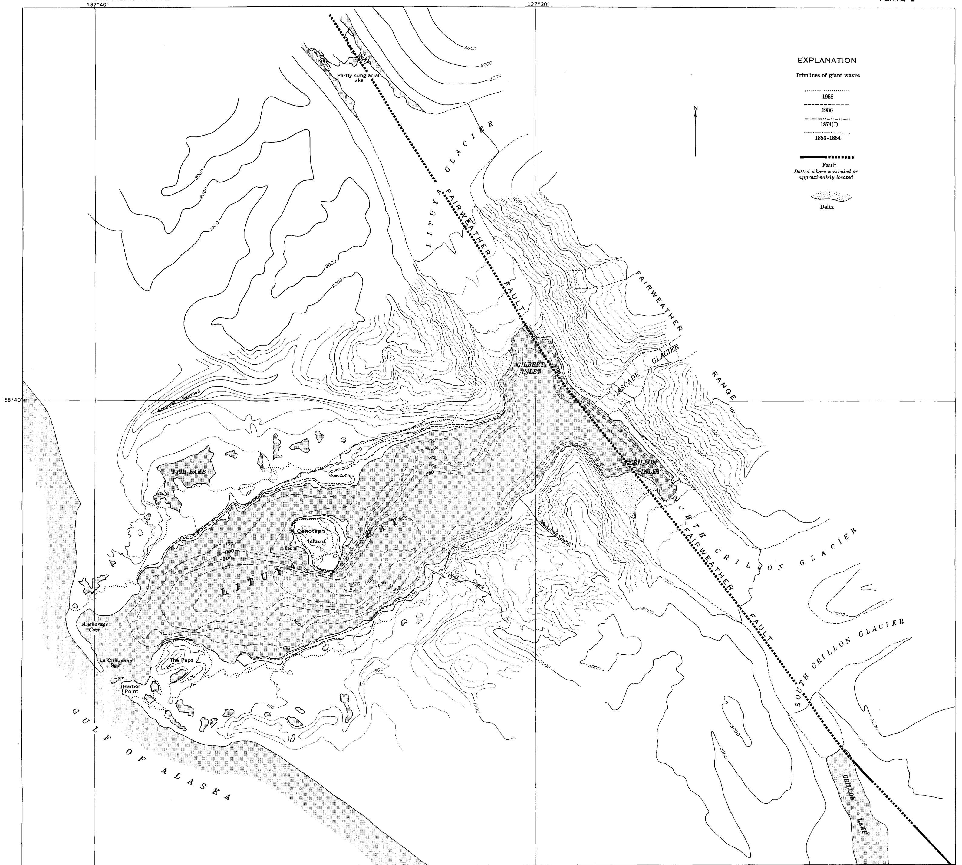
MAP OF LITUYA BAY AND ADJOINING AREA, SHOWING SUBAERIAL AND SUBMARINE TOPOGRAPHY, TRACE OF FAIRWEATHER FAULT AND TRIMLINES OF KNOWN GIANT WAVES AS MAPPED IN THE FIELD AND FROM PHOTOGRAPHS
