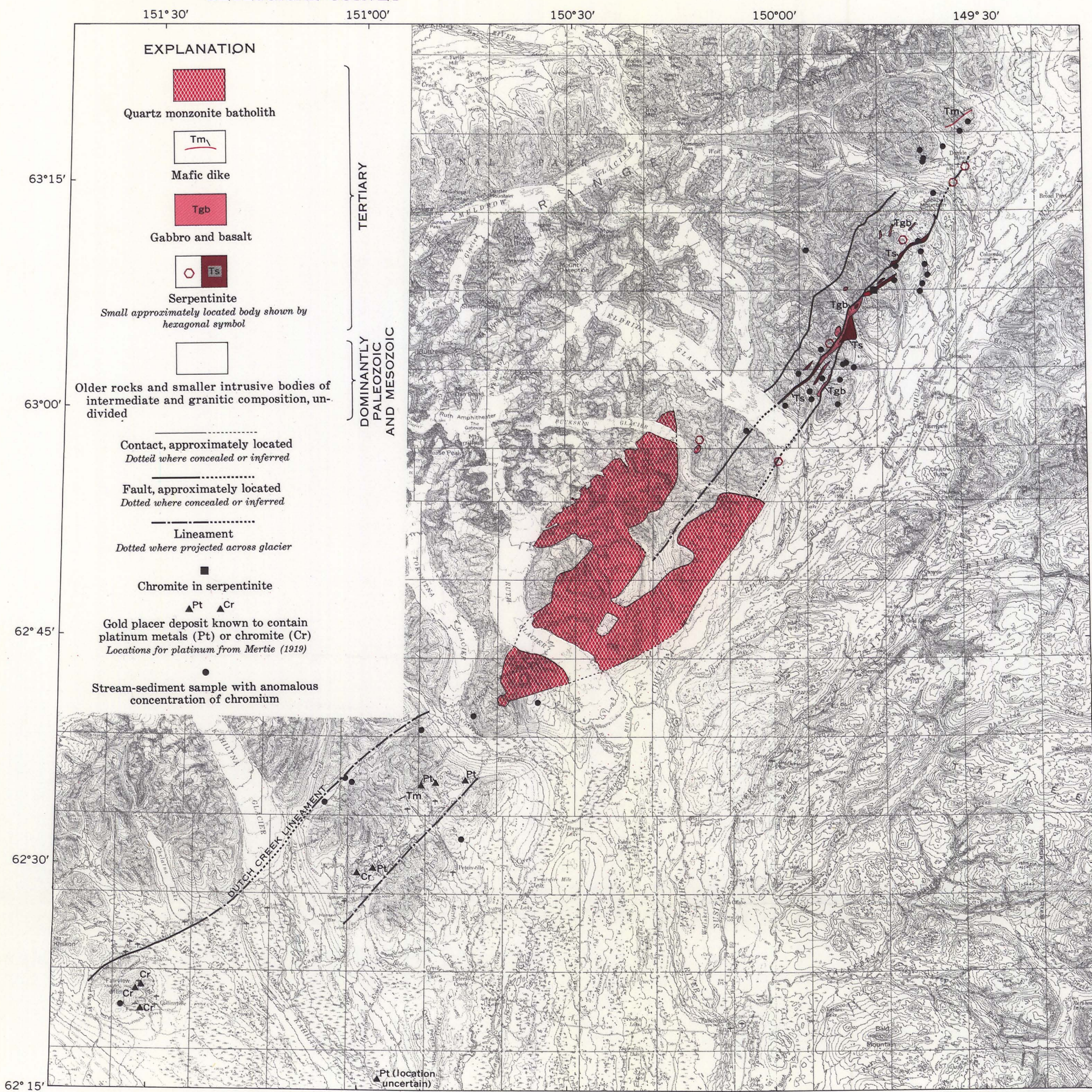
MAFIC AND ULTRAMAFIC ROCKS, PLATINUM, AND CHROMIUM
