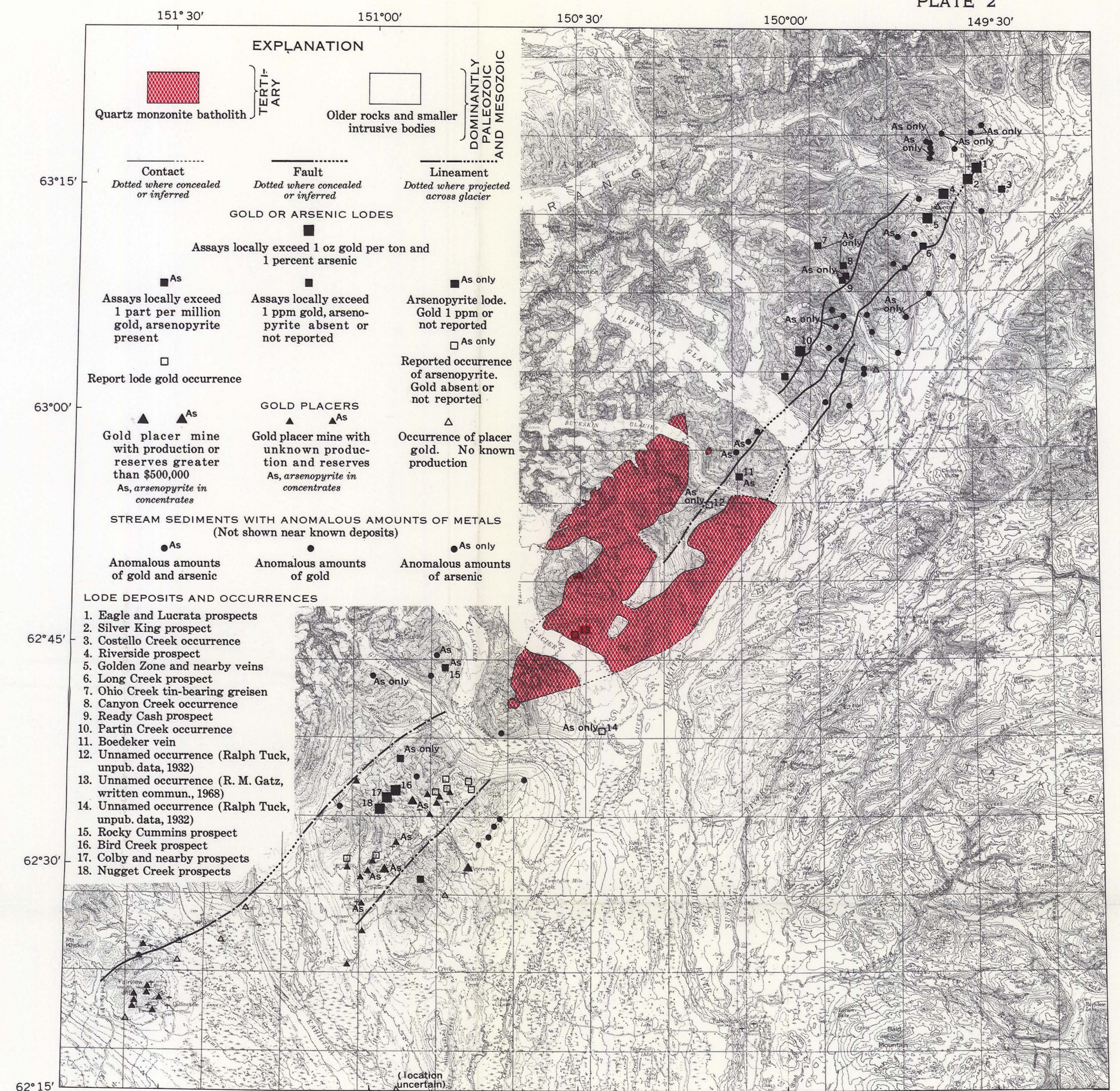
GOLD AND ARSENIC
