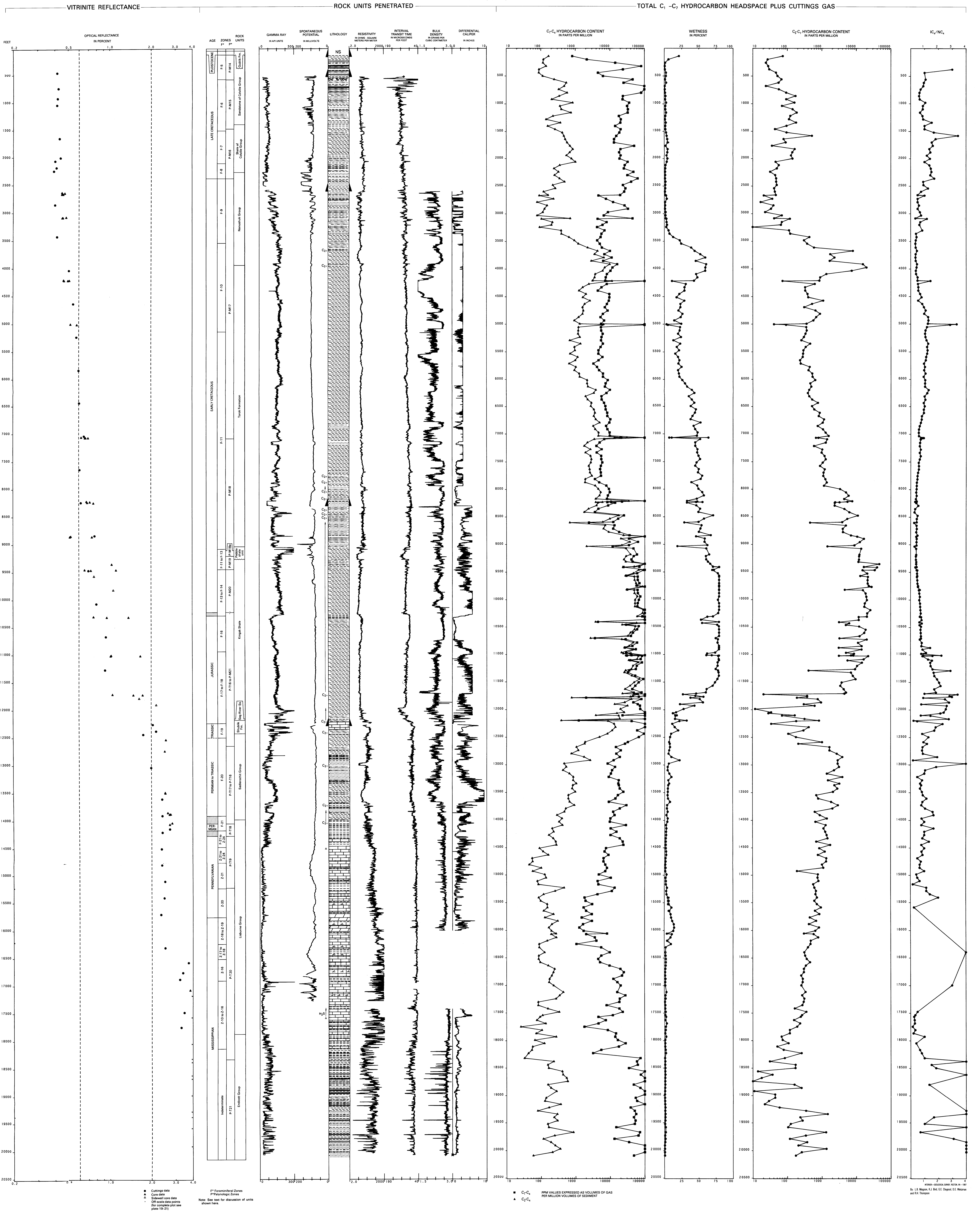
VITRINITE REFLECTANCE AND HYDROCARBON DATA FOR INIGOK NO. 1 WELL, NORTH SLOPE, ALASKA
