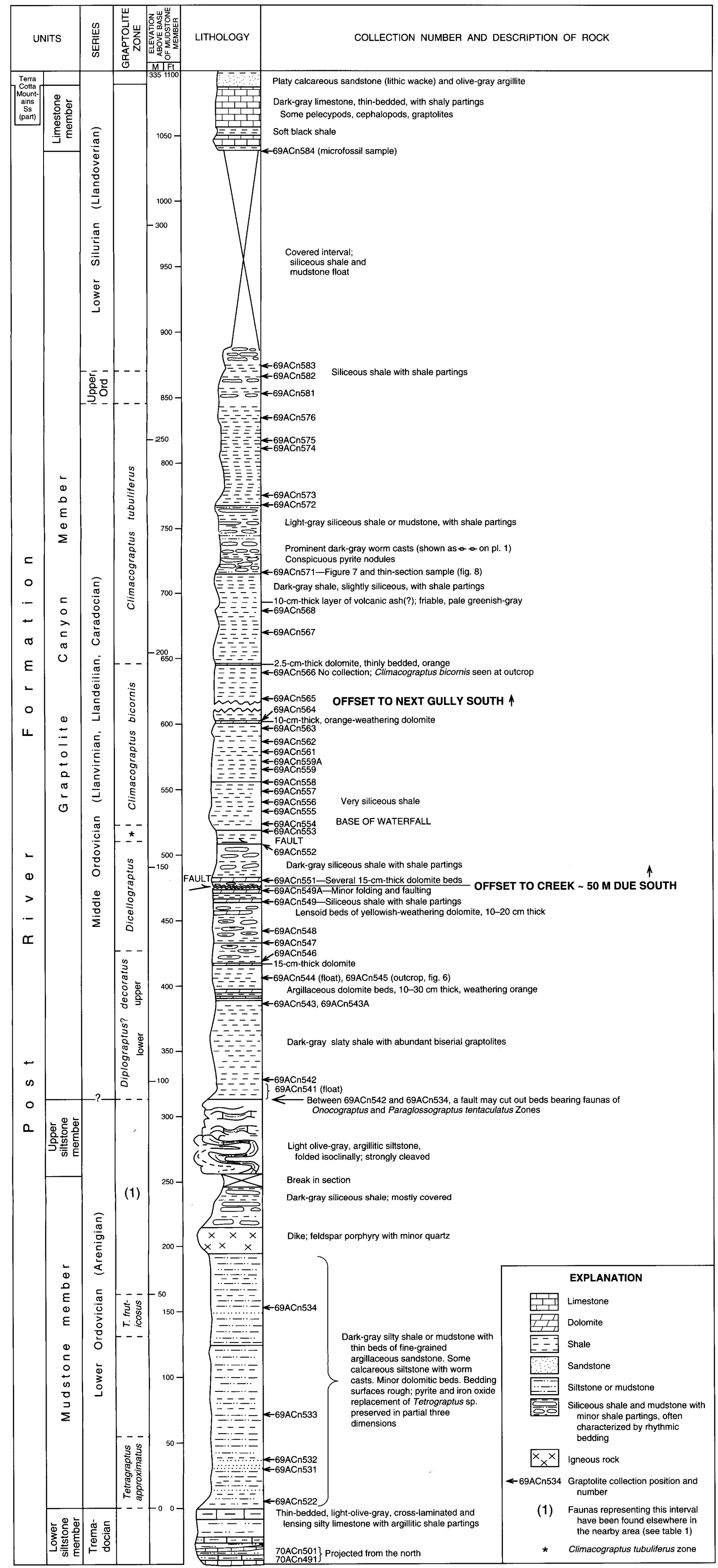
B. MEASURED SECTION OF THE TYPE POST RIVER FORMATION, TERRA COTTA MOUNTAINS, ALASKA, SHOWING GRAPTOLITE HORIZONS
