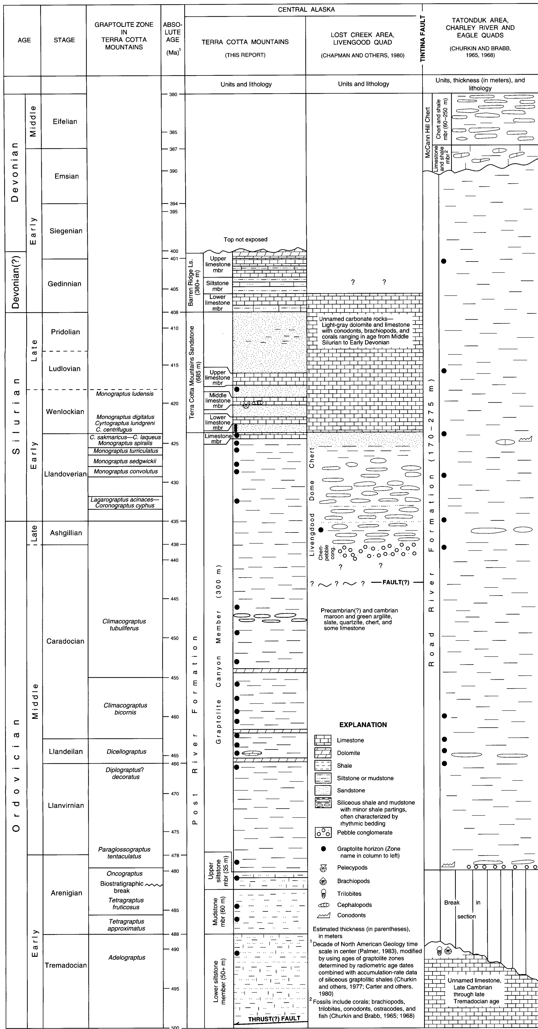
A. CORRELATION CHART OF GRAPTOLITE-RICH ARGILLACEOUS SUCCESSIONS IN CENTRAL ALASKA
