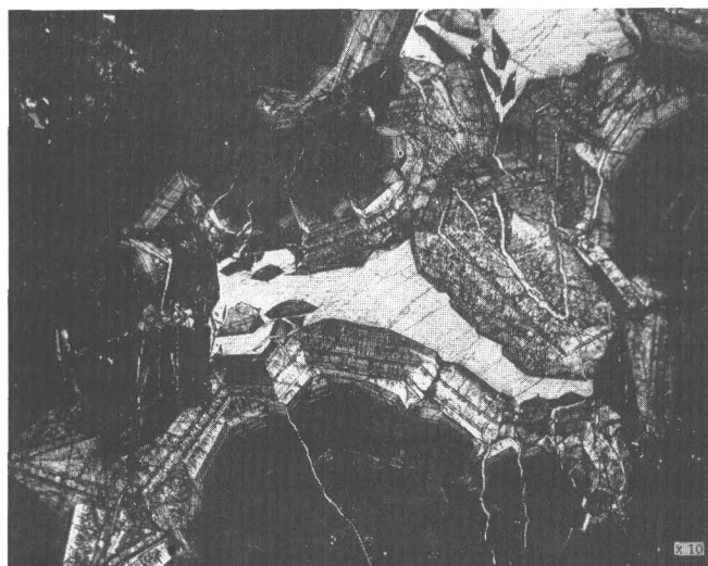
FIGURE 30.—Zoned garnets characteristic of Jumbo mine, Alaska. Crossed nicols.
