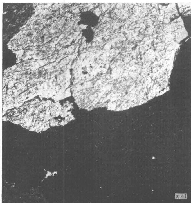
FIGURE 12.—Coarse-grained magnetite replacing diopside, Magnetite Cliff, Jumbo basin, Alaska. Crossed nicols.
