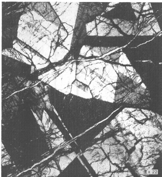
FIGURE 24.—Coarsely twinned garnet characteristic of upper magnetite bodies. Garnets are cut by fine veinlets of calcite, Jumbo basin, Alaska. Crossed nicols.
