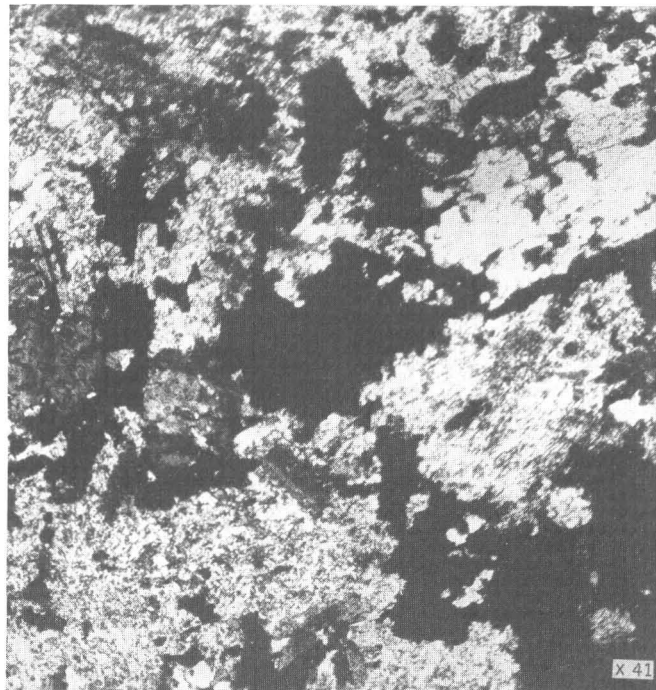
FIGURE 17.—Sericitized feldspar of intrusive rock followed by clinozoisite (lath-shaped twinned crystals), diopside (light crystals), and garnet (black irregular areas), Magnetite Cliff, Jumbo basin, Alaska. Crossed nicols.
