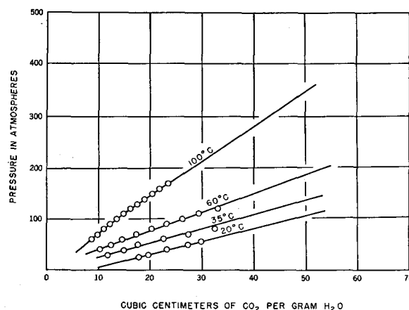
FIGURE 39.—Solubility isotherms of CO 2 in water.
