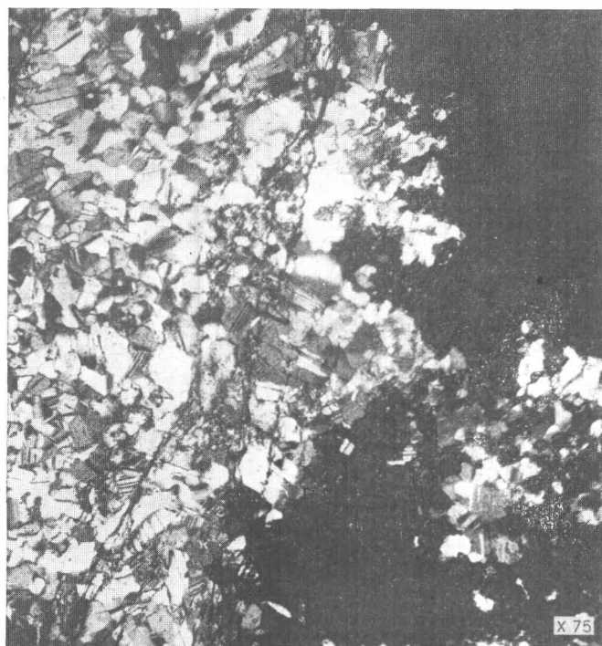
FIGURE 14.—Plagioclase lath broken down to an aggregate of many small plagioclase crystals of higher anorthite content, garnet surrounding and replacing feldspar, Magnetite Cliff, Jumbo basin, Alaska. Crossed nicols.
