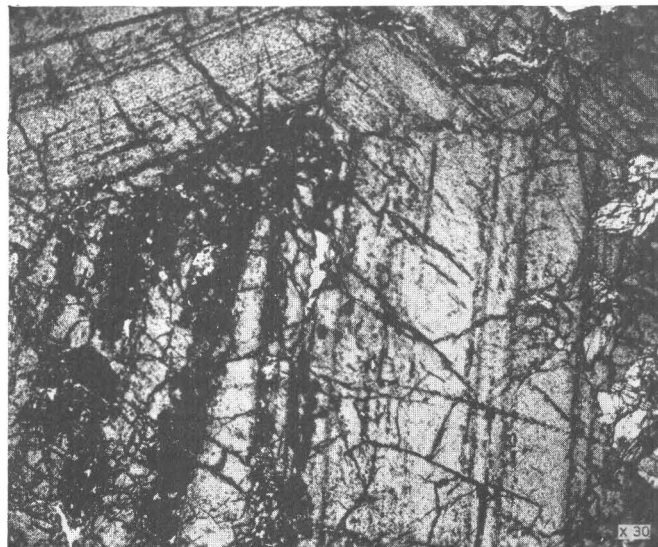
FIGURE 13.—Zoned isotropic garnet with included diopside grains. Chalcopyrite (black) is preferentially replacing certain garnet zones, Magnetite Cliff, Jumbo basin, Alaska. Plane light.
