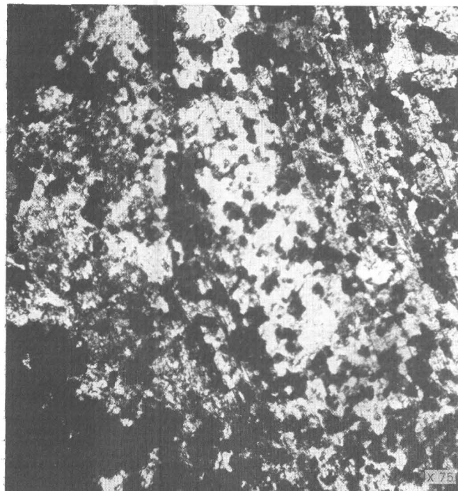
FIGURE 15.—Fine-grained garnet (black) replacing orthoclase feldspar, Magnetite Cliff, Jumbo basin, Alaska. Crossed nicols.
