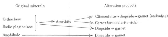
FIGURE 18.—Sequence of replacement in the endomorphosed zone.
