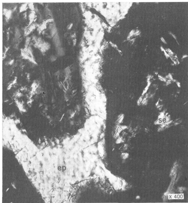
FIGURE 34.—Feldspar of augite monzonite replaced by sericite and epidote, Jumbo mine, Alaska. Epidote, ep; sericite, se. Crossed nicols.
