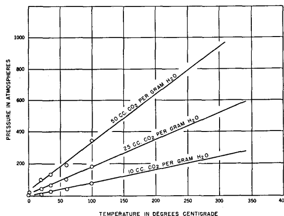
FIGURE 40.—Curves of solubility of CO 2 in H 2 O at various temperatures and pressures
