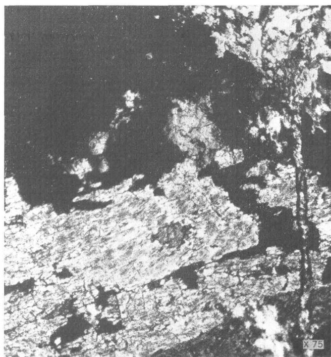
FIGURE 16.—Altered granodiorite, showing garnet (black) replacing diopside and clinozoisite, Magnetite Cliff, Jumbo basin, Alaska. Crossed nicols.
