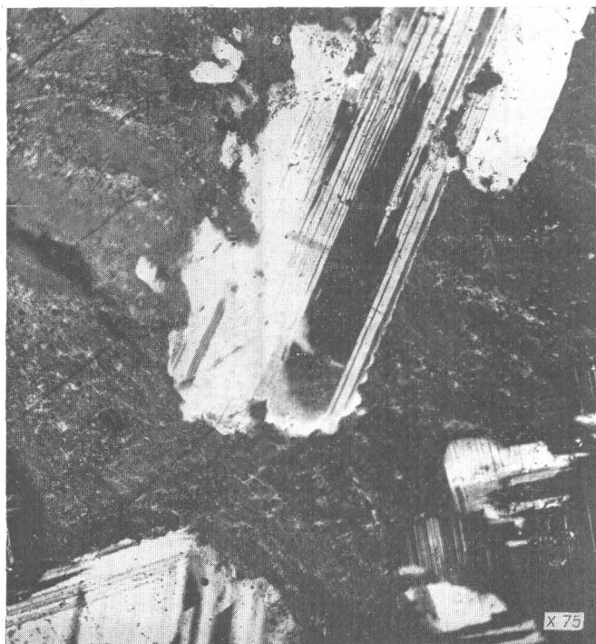
FIGURE 5.—Residual crystals of plagioclase surrounded by orthoclase, Magnetite Cliff, Jumbo basin, Alaska. Crossed nicols.
