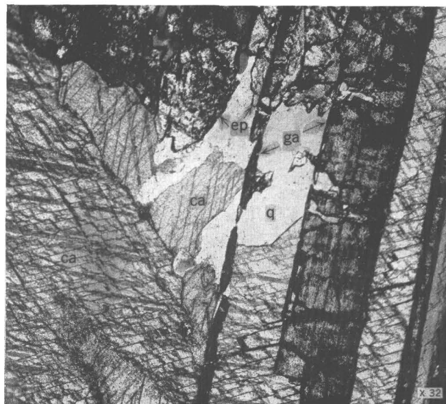
FIGURE 31.—Zoned anisotropic garnet replaced by epidote, quartz, and calcite. Replacement is preferential along certain zones, Jumbo mine, Alaska. Quartz, q; garnet, ga; epidote, ep; calcite, ca. Crossed nicols.
