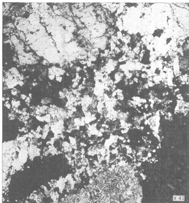
FIGURE 20.—Diopside rock, showing dual grain size characteristic of diopside formed by replacement of intrusive rock, Magnetite Cliff, Jumbo basin, Alaska. Crossed nicols.
