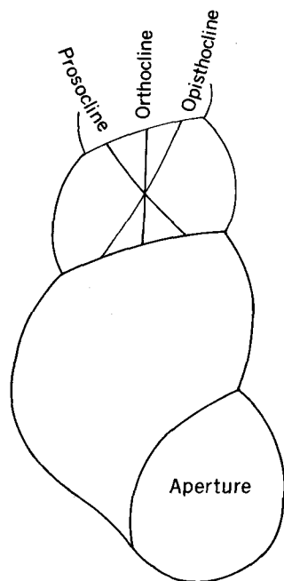
FIGURE 26.—Schematic representation of terms for direction of growth lines.
