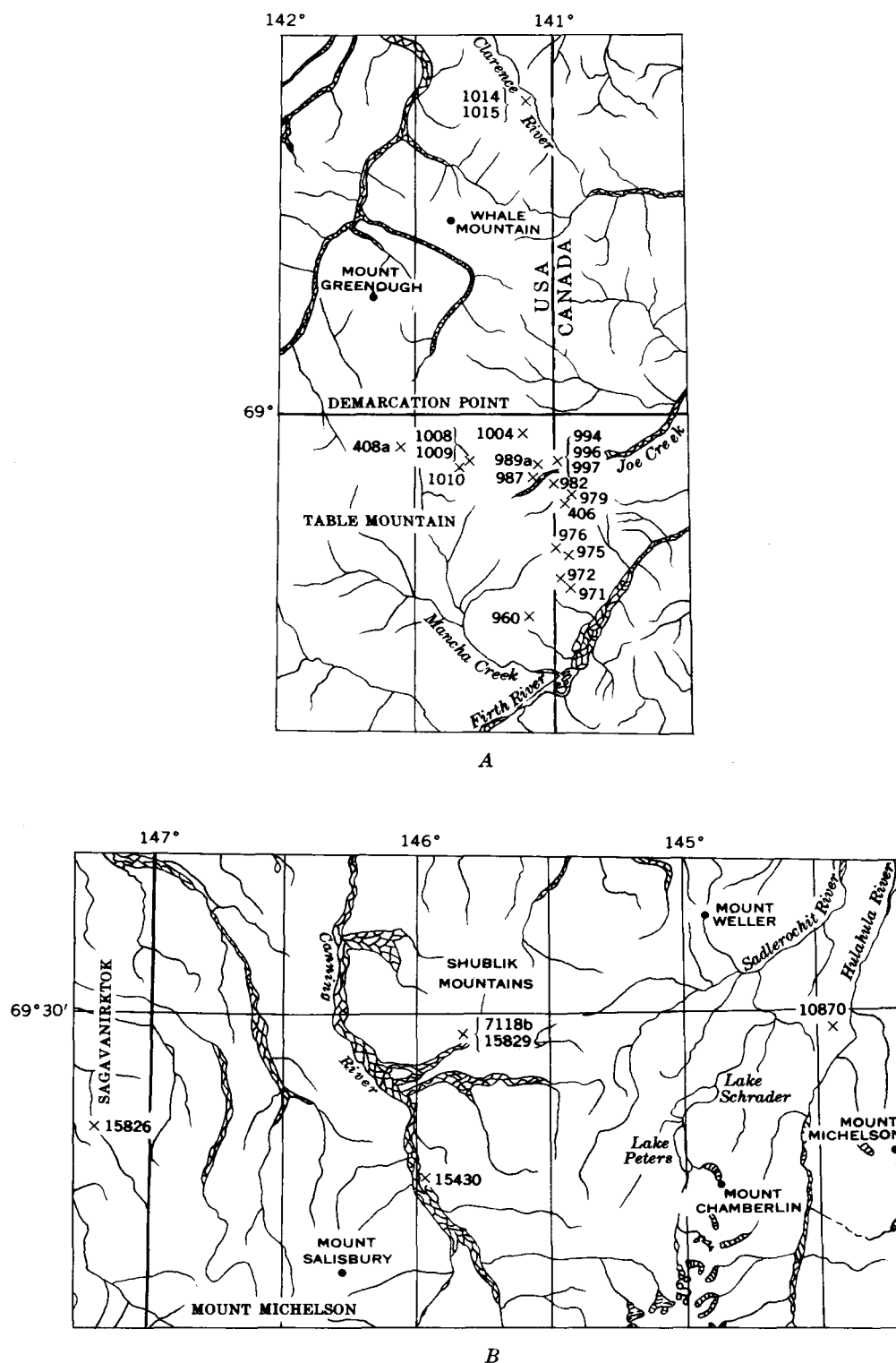
FIGURE 29.—Fossil-collecting localities in parts of the Demarcation Point and Table Mountain quadrangles, Alaska, and adjacent parts of Canada (A) and the Sagavanirktok and Mount Michelson quadrangles, Alaska (B).
