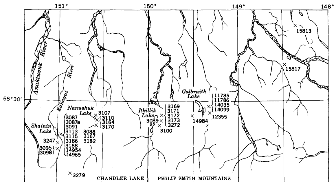
FIGURE 28.—Fossil-collecting localities in parts of the Killik River and Chandler Lake quadrangles (A) and the Chandler Lake and Philip Smith Mountains quadrangles (B), Alaska.
